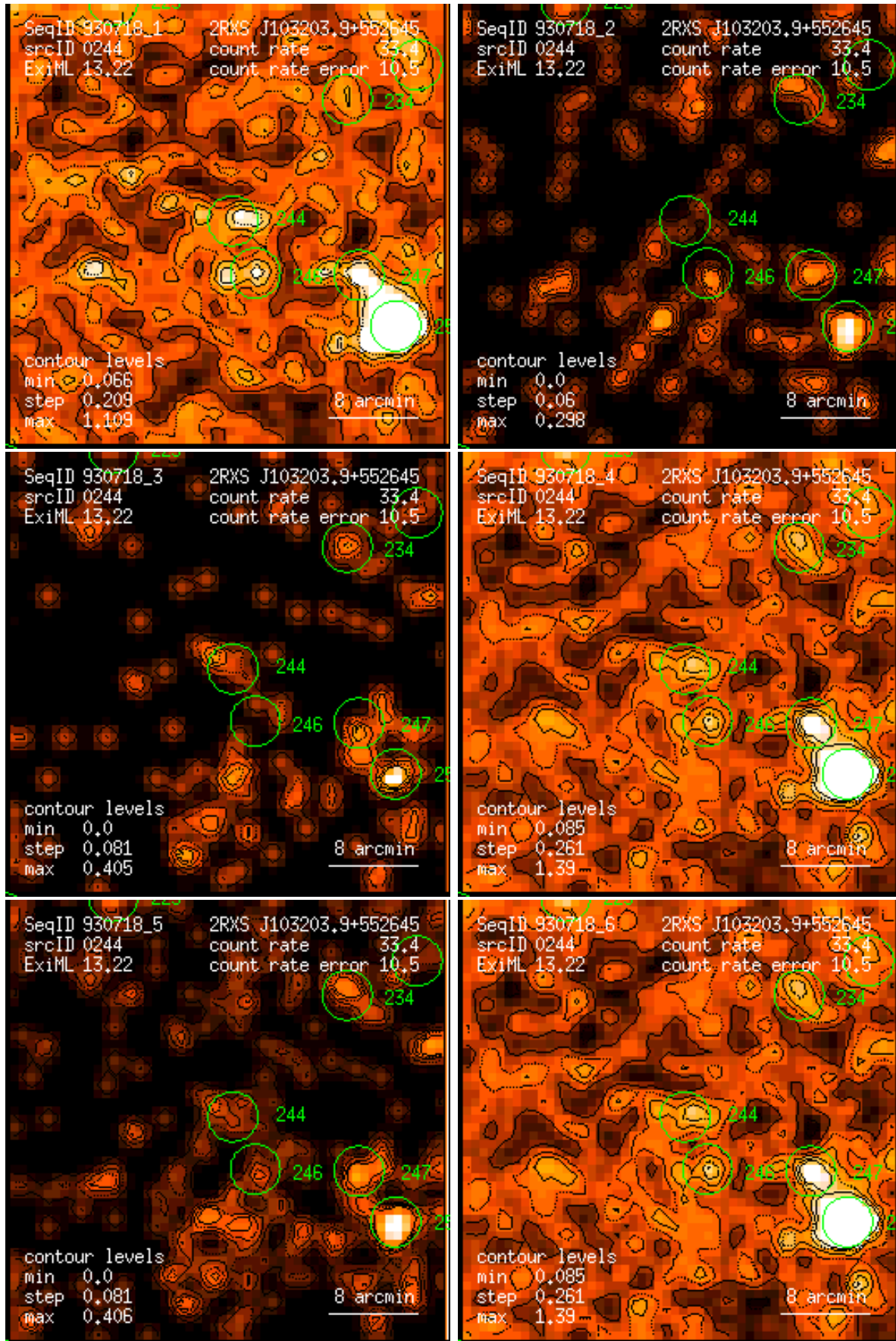
Figure 244: RASS 930718: detection 0244: band rate images, Gaussian filter: (1) PSPC channels 11 – 41, (2) 52 – 90, (3) 91 – 201, (4) 11 – 235, (5) 52 – 201, (6) 11 – 201. Broad band rates in counts/ks. Band rate contour levels in counts/ks/arcmin 2 .
