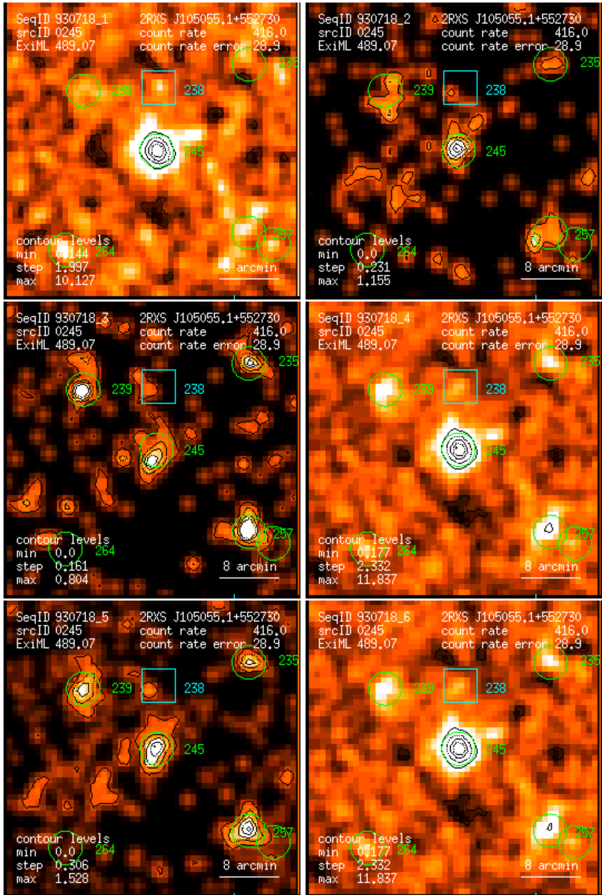
Figure 245: RASS 930718: detection 0245: band rate images, Gaussian filter: (1) PSPC channels 11 – 41, (2) 52 – 90, (3) 91 – 201, (4) 11 – 235, (5) 52 – 201, (6) 11 – 201. Broad band rates in counts/ks. Band rate contour levels in counts/ks/arcmin 2 .
