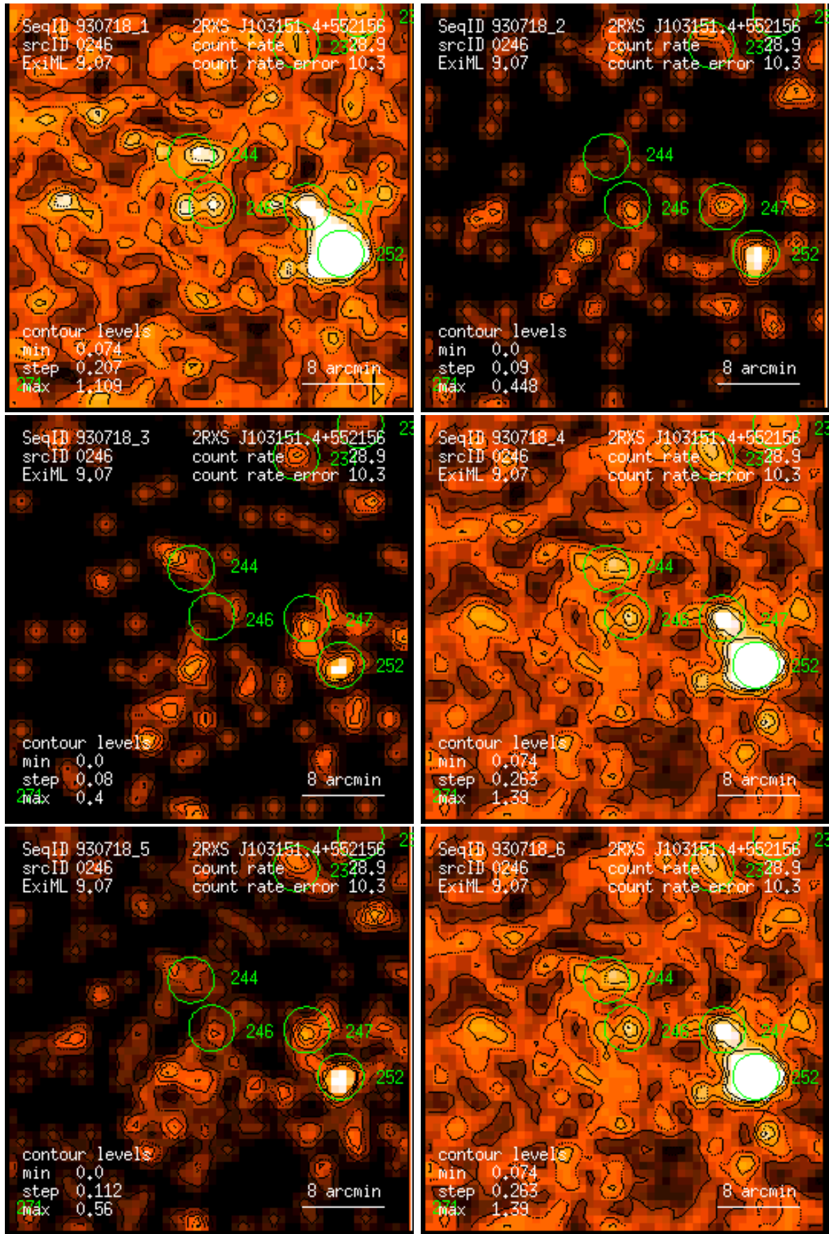
Figure 246: RASS 930718: detection 0246: band rate images, Gaussian filter: (1) PSPC channels 11 – 41, (2) 52 – 90, (3) 91 – 201, (4) 11 – 235, (5) 52 – 201, (6) 11 – 201. Broad band rates in counts/ks. Band rate contour levels in counts/ks/arcmin 2 .
