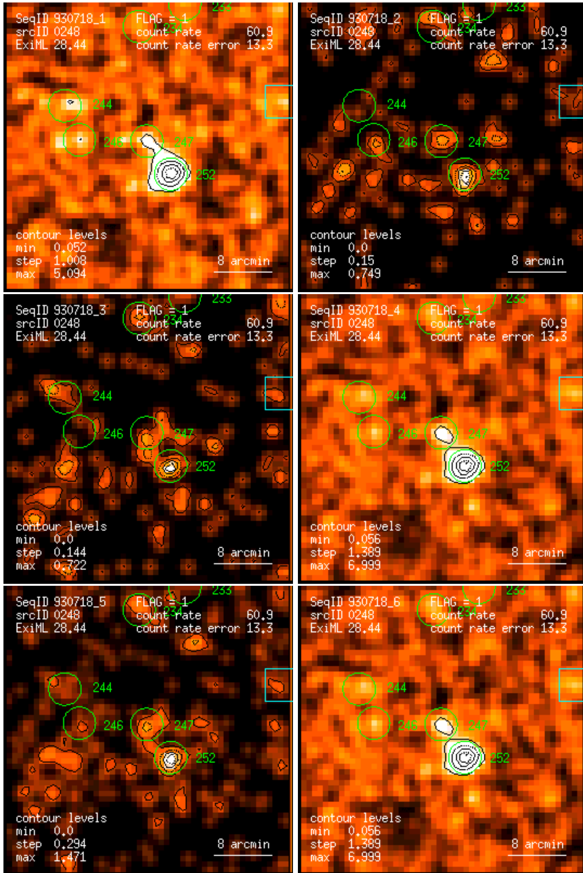
Figure 248: RASS 930718: detection 0248: band rate images, Gaussian filter: (1) PSPC channels 11 – 41, (2) 52 – 90, (3) 91 – 201, (4) 11 – 235, (5) 52 – 201, (6) 11 – 201. Broad band rates in counts/ks. Band rate contour levels in counts/ks/arcmin 2 .
