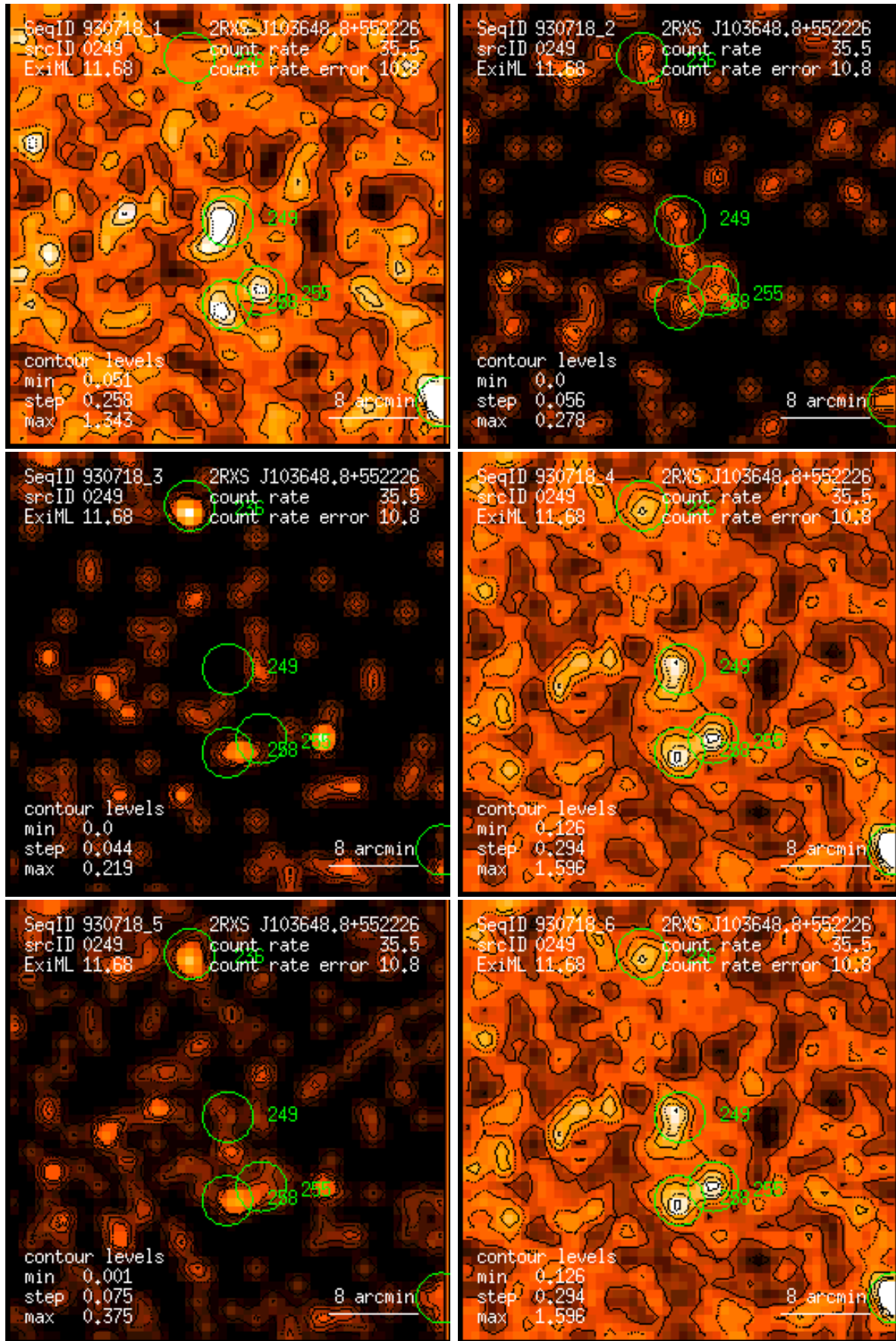
Figure 249: RASS 930718: detection 0249: band rate images, Gaussian filter: (1) PSPC channels 11 – 41, (2) 52 – 90, (3) 91 – 201, (4) 11 – 235, (5) 52 – 201, (6) 11 – 201. Broad band rates in counts/ks. Band rate contour levels in counts/ks/arcmin 2 .
