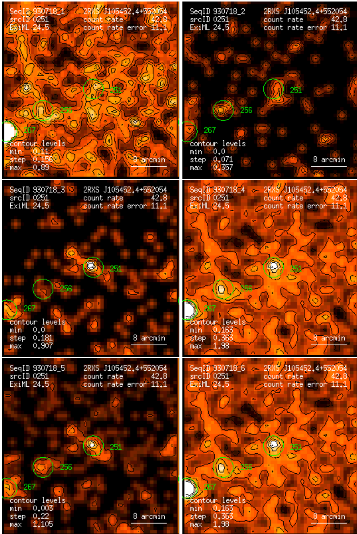
Figure 251: RASS 930718: detection 0251: band rate images, Gaussian filter: (1) PSPC channels 11 – 41, (2) 52 – 90, (3) 91 – 201, (4) 11 – 235, (5) 52 – 201, (6) 11 – 201. Broad band rates in counts/ks. Band rate contour levels in counts/ks/arcmin 2 .
