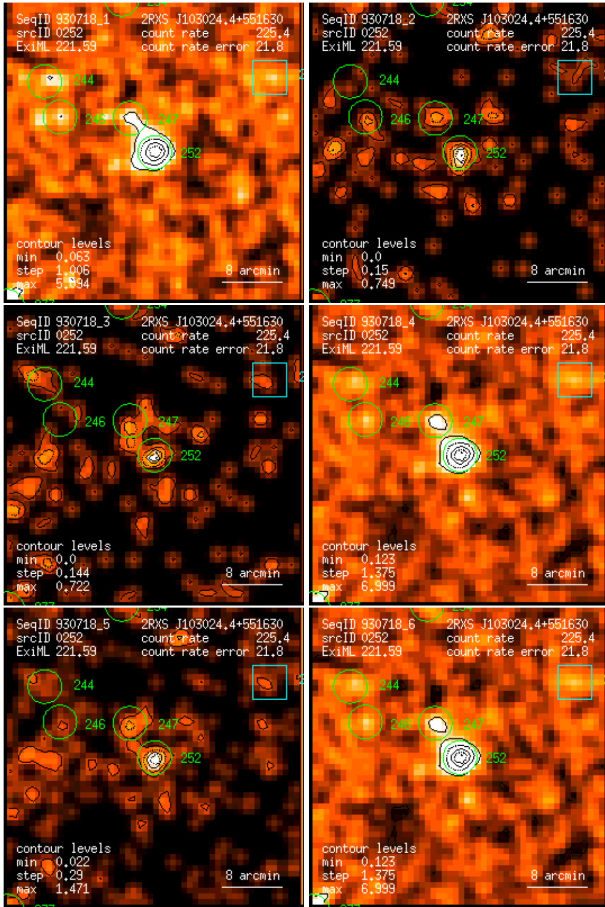
Figure 252: RASS 930718: detection 0252: band rate images, Gaussian filter: (1) PSPC channels 11 – 41, (2) 52 – 90, (3) 91 – 201, (4) 11 – 235, (5) 52 – 201, (6) 11 – 201. Broad band rates in counts/ks. Band rate contour levels in counts/ks/arcmin 2 .
