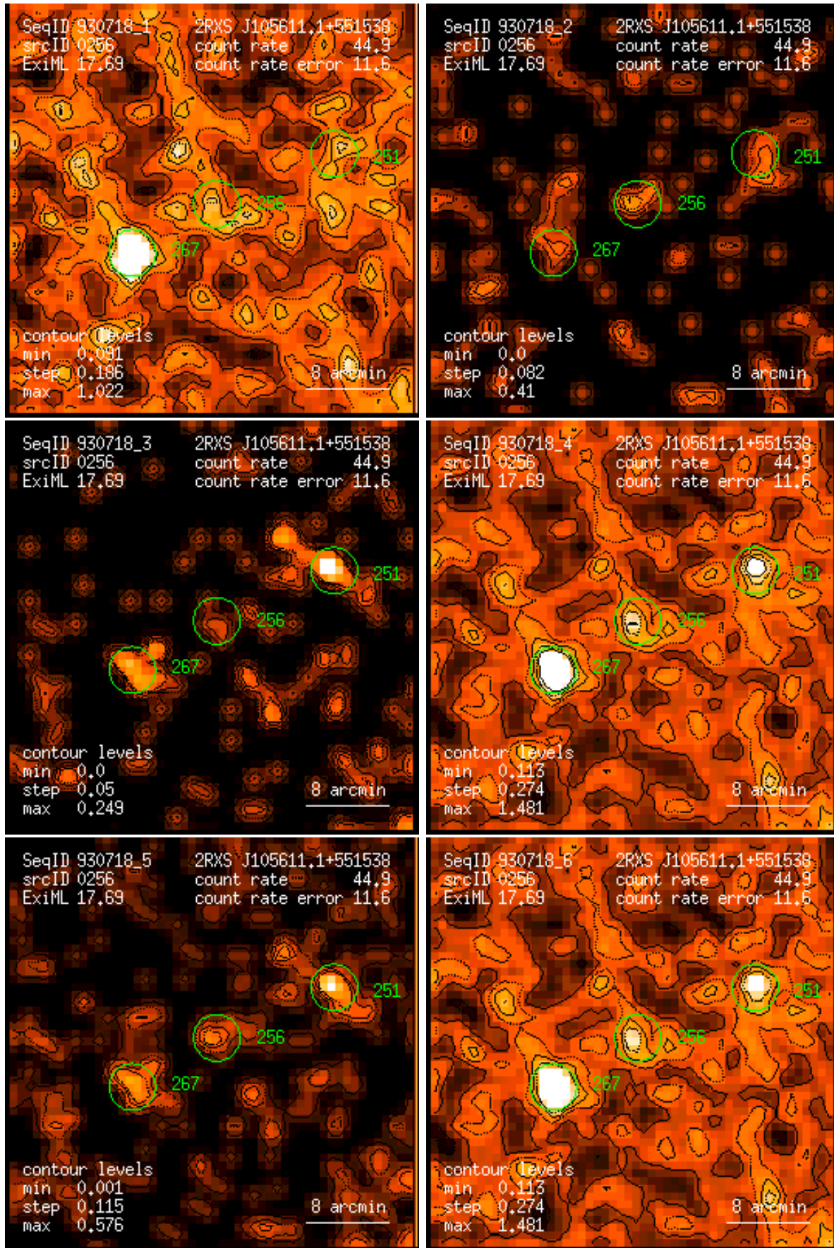
Figure 256: RASS 930718: detection 0256: band rate images, Gaussian filter: (1) PSPC channels 11 – 41, (2) 52 – 90, (3) 91 – 201, (4) 11 – 235, (5) 52 – 201, (6) 11 – 201. Broad band rates in counts/ks. Band rate contour levels in counts/ks/arcmin 2 .
