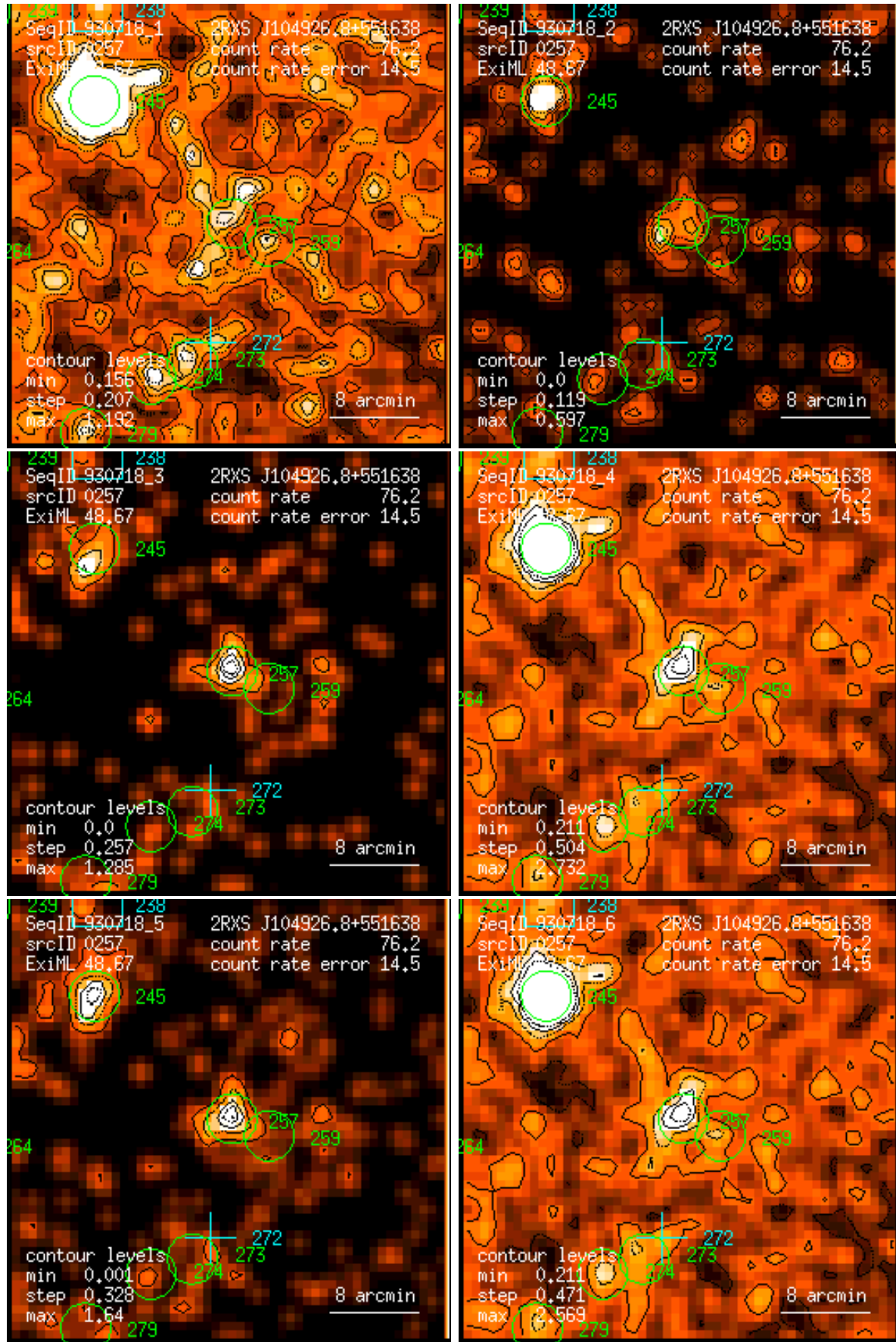
Figure 257: RASS 930718: detection 0257: band rate images, Gaussian filter: (1) PSPC channels 11 – 41, (2) 52 – 90, (3) 91 – 201, (4) 11 – 235, (5) 52 – 201, (6) 11 – 201. Broad band rates in counts/ks. Band rate contour levels in counts/ks/arcmin 2 .
