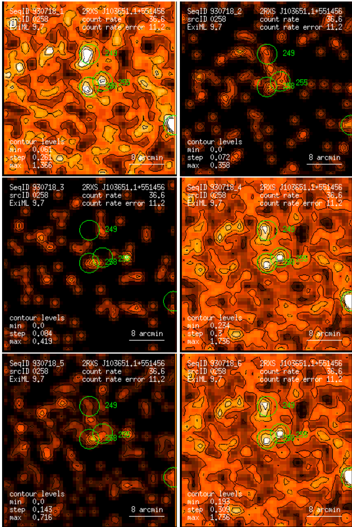
Figure 258: RASS 930718: detection 0258: band rate images, Gaussian filter: (1) PSPC channels 11 – 41, (2) 52 – 90, (3) 91 – 201, (4) 11 – 235, (5) 52 – 201, (6) 11 – 201. Broad band rates in counts/ks. Band rate contour levels in counts/ks/arcmin 2 .
