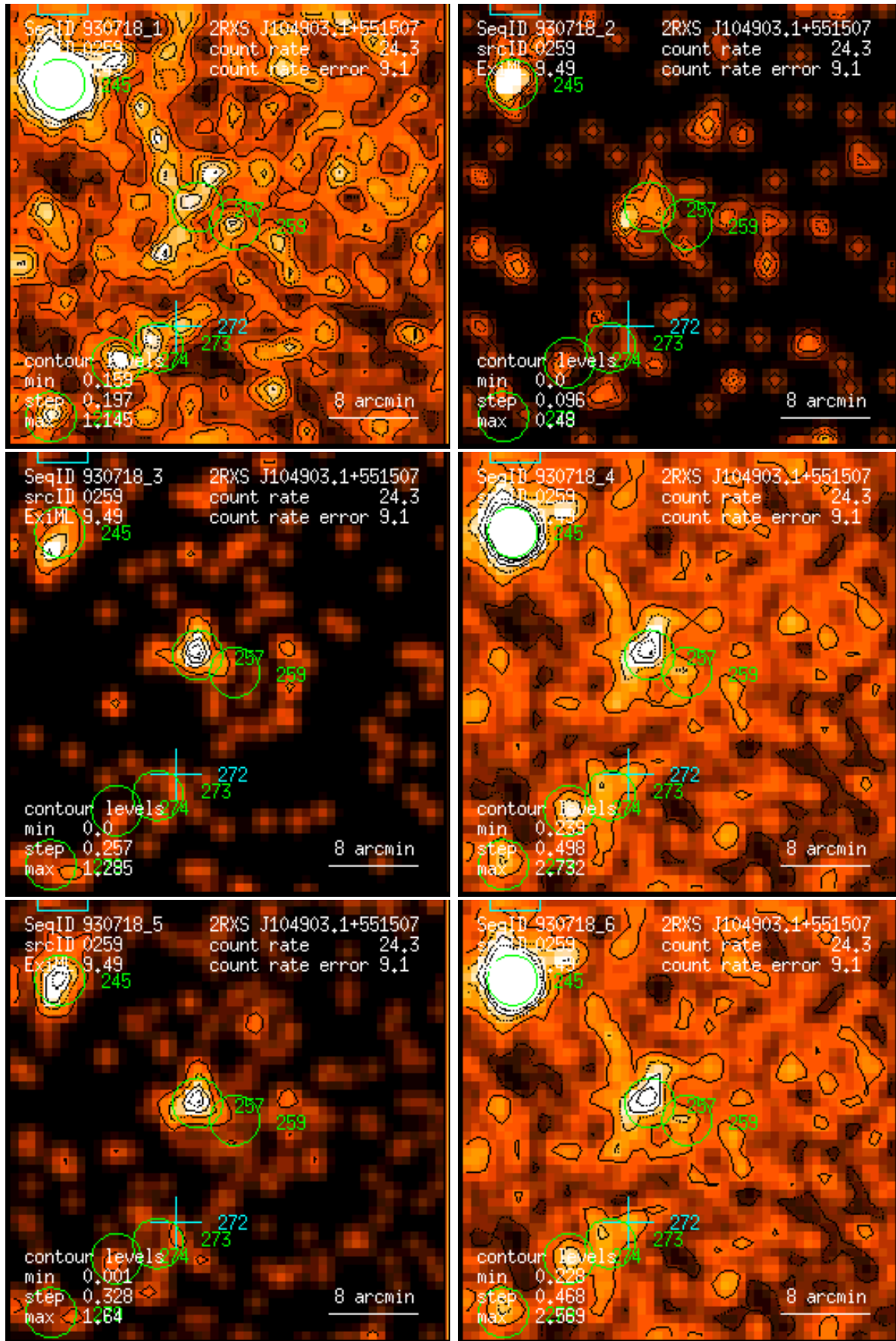
Figure 259: RASS 930718: detection 0259: band rate images, Gaussian filter: (1) PSPC channels 11 – 41, (2) 52 – 90, (3) 91 – 201, (4) 11 – 235, (5) 52 – 201, (6) 11 – 201. Broad band rates in counts/ks. Band rate contour levels in counts/ks/arcmin 2 .
