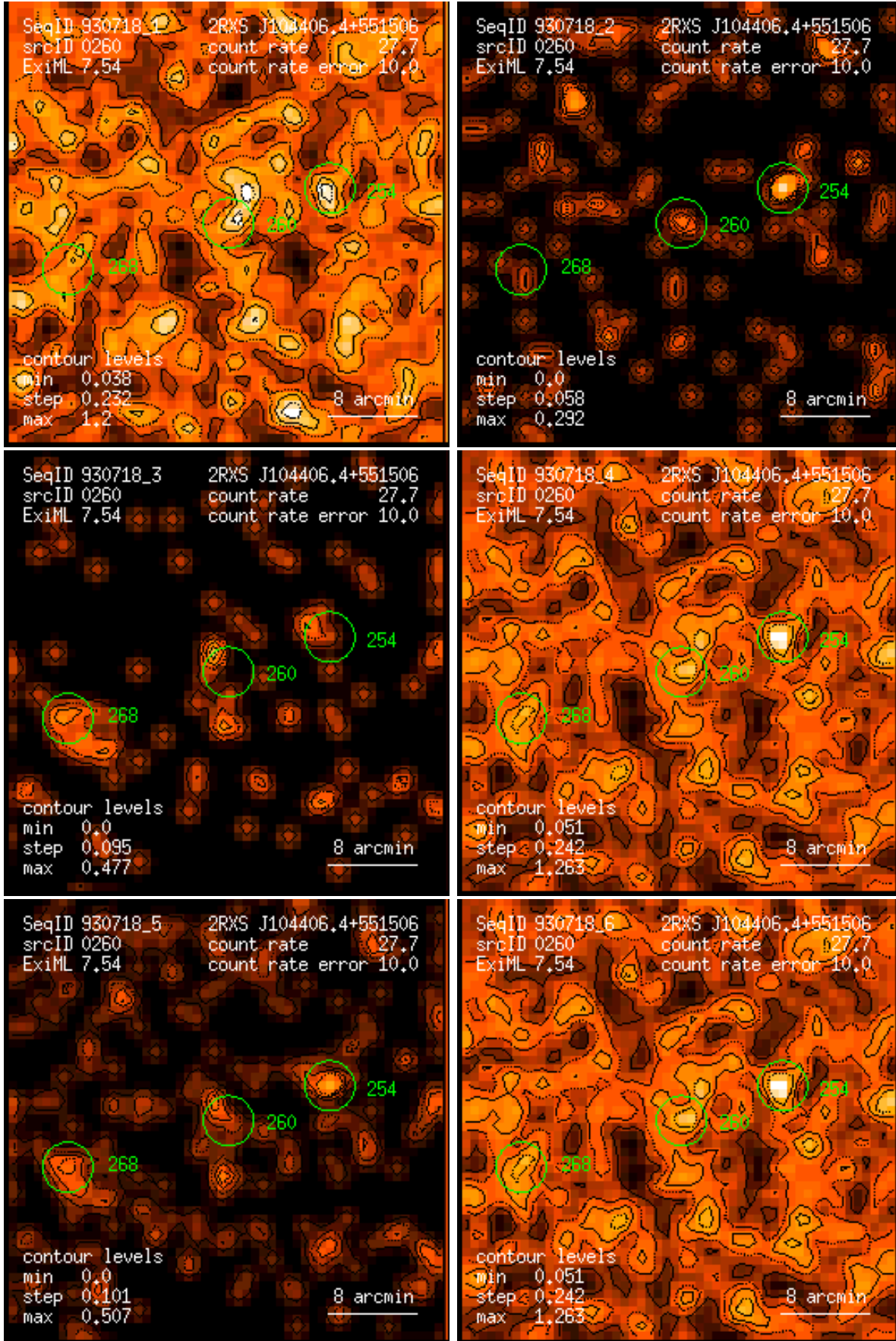
Figure 260: RASS 930718: detection 0260: band rate images, Gaussian filter: (1) PSPC channels 11 – 41, (2) 52 – 90, (3) 91 – 201, (4) 11 – 235, (5) 52 – 201, (6) 11 – 201. Broad band rates in counts/ks. Band rate contour levels in counts/ks/arcmin 2 .
