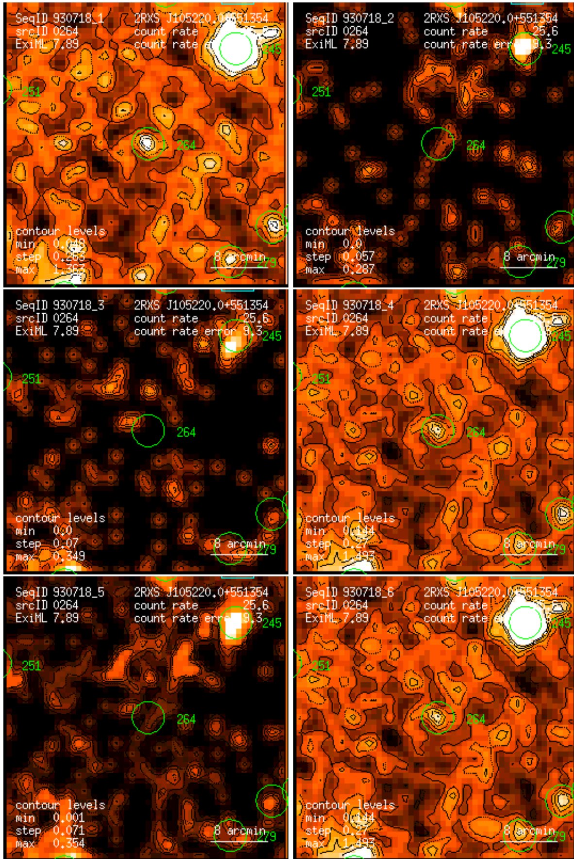
Figure 264: RASS 930718: detection 0264: band rate images, Gaussian filter: (1) PSPC channels 11 – 41, (2) 52 – 90, (3) 91 – 201, (4) 11 – 235, (5) 52 – 201, (6) 11 – 201. Broad band rates in counts/ks. Band rate contour levels in counts/ks/arcmin 2 .
