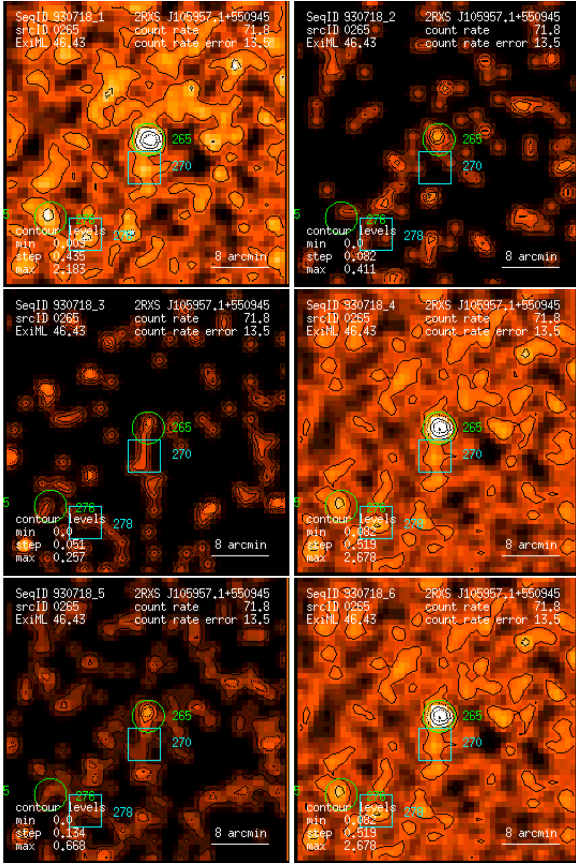
Figure 265: RASS 930718: detection 0265: band rate images, Gaussian filter: (1) PSPC channels 11 – 41, (2) 52 – 90, (3) 91 – 201, (4) 11 – 235, (5) 52 – 201, (6) 11 – 201. Broad band rates in counts/ks. Band rate contour levels in counts/ks/arcmin 2 .
