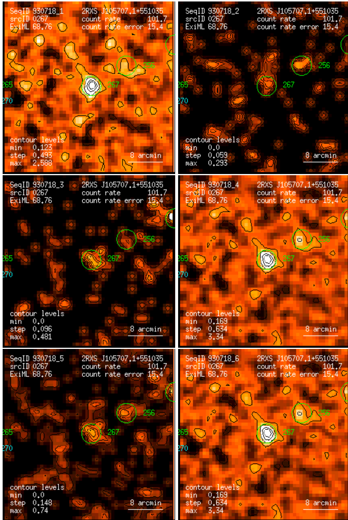
Figure 267: RASS 930718: detection 0267: band rate images, Gaussian filter: (1) PSPC channels 11 – 41, (2) 52 – 90, (3) 91 – 201, (4) 11 – 235, (5) 52 – 201, (6) 11 – 201. Broad band rates in counts/ks. Band rate contour levels in counts/ks/arcmin 2 .
