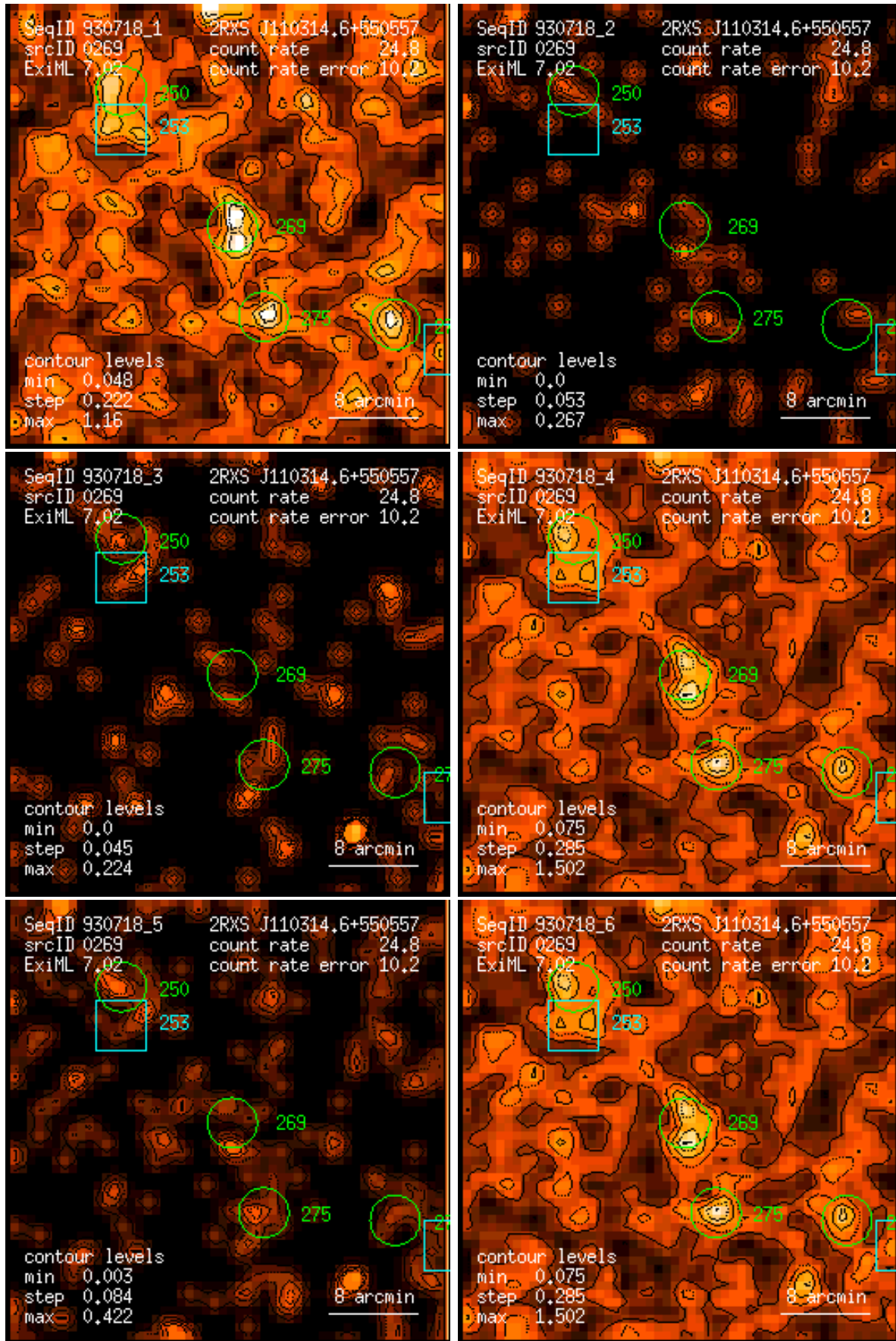
Figure 269: RASS 930718: detection 0269: band rate images, Gaussian filter: (1) PSPC channels 11 – 41, (2) 52 – 90, (3) 91 – 201, (4) 11 – 235, (5) 52 – 201, (6) 11 – 201. Broad band rates in counts/ks. Band rate contour levels in counts/ks/arcmin 2 .
