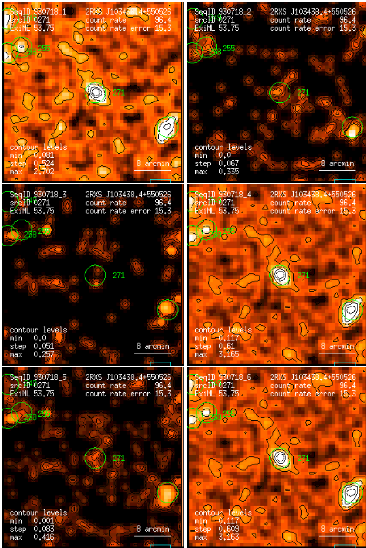
Figure 271: RASS 930718: detection 0271: band rate images, Gaussian filter: (1) PSPC channels 11 – 41, (2) 52 – 90, (3) 91 – 201, (4) 11 – 235, (5) 52 – 201, (6) 11 – 201. Broad band rates in counts/ks. Band rate contour levels in counts/ks/arcmin 2 .
