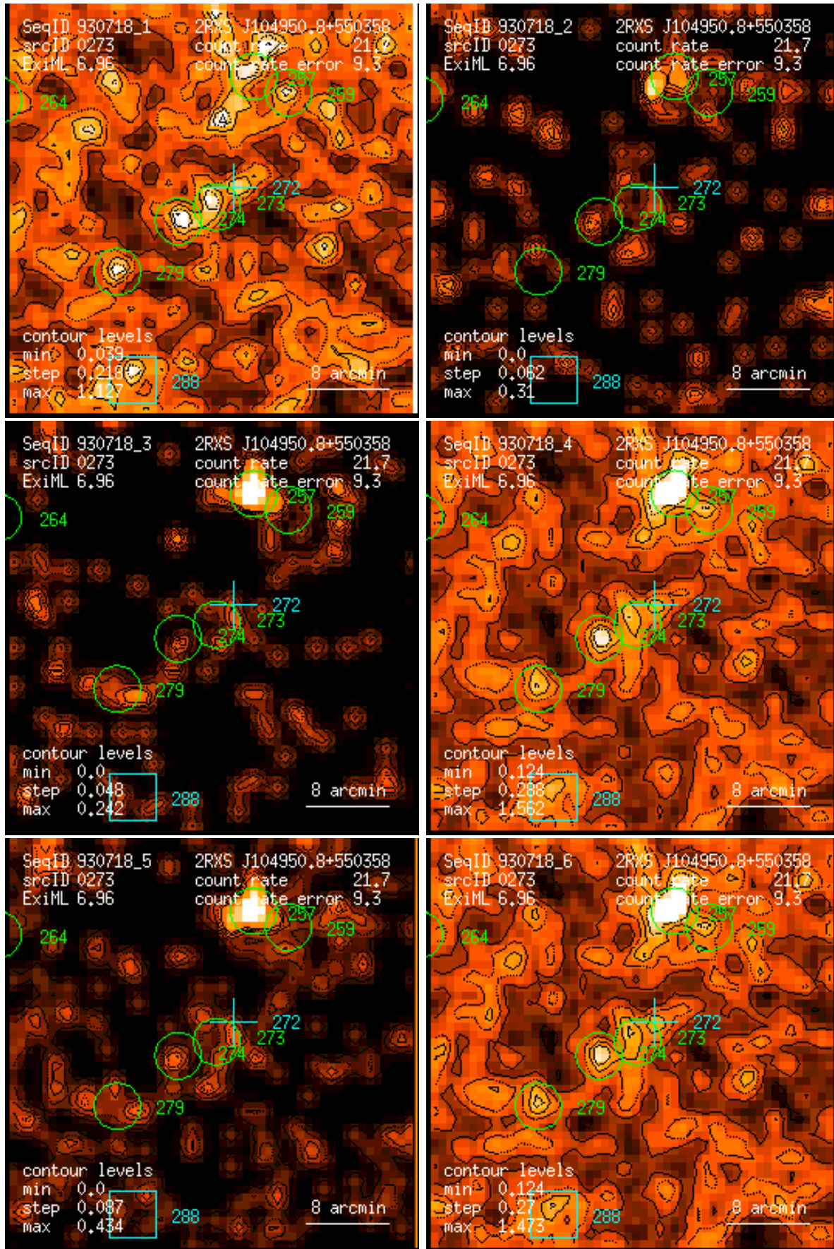
Figure 273: RASS 930718: detection 0273: band rate images, Gaussian filter: (1) PSPC channels 11 – 41, (2) 52 – 90, (3) 91 – 201, (4) 11 – 235, (5) 52 – 201, (6) 11 – 201. Broad band rates in counts/ks. Band rate contour levels in counts/ks/arcmin 2 .
