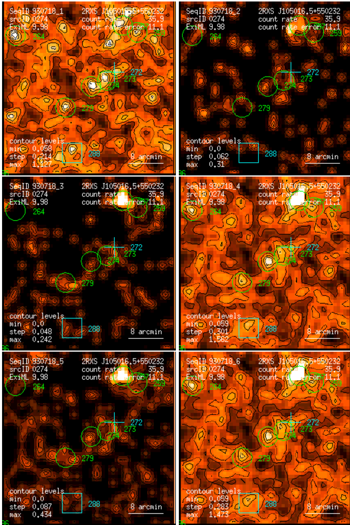
Figure 274: RASS 930718: detection 0274: band rate images, Gaussian filter: (1) PSPC channels 11 – 41, (2) 52 – 90, (3) 91 – 201, (4) 11 – 235, (5) 52 – 201, (6) 11 – 201. Broad band rates in counts/ks. Band rate contour levels in counts/ks/arcmin 2 .
