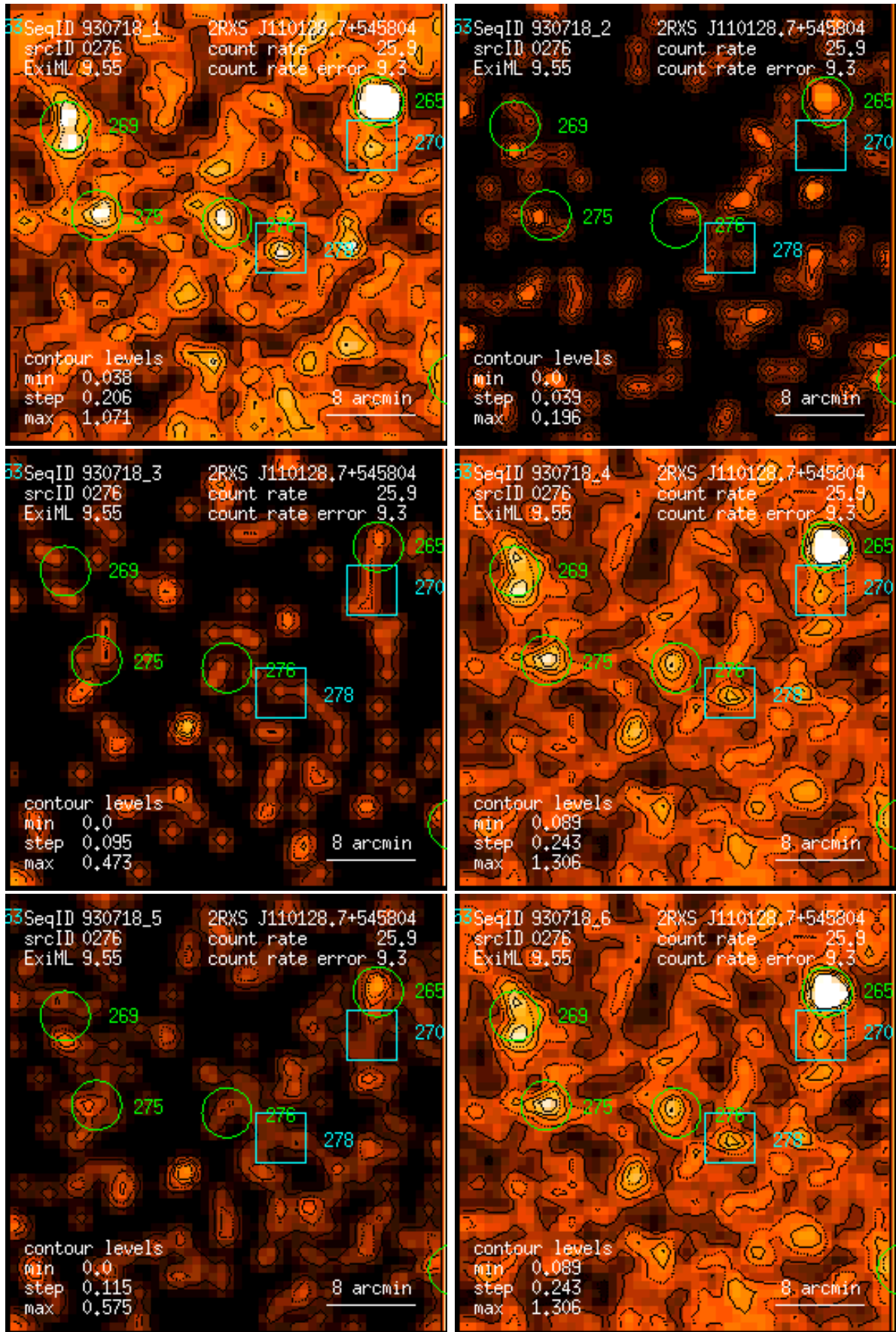
Figure 276: RASS 930718: detection 0276: band rate images, Gaussian filter: (1) PSPC channels 11 – 41, (2) 52 – 90, (3) 91 – 201, (4) 11 – 235, (5) 52 – 201, (6) 11 – 201. Broad band rates in counts/ks. Band rate contour levels in counts/ks/arcmin 2 .
