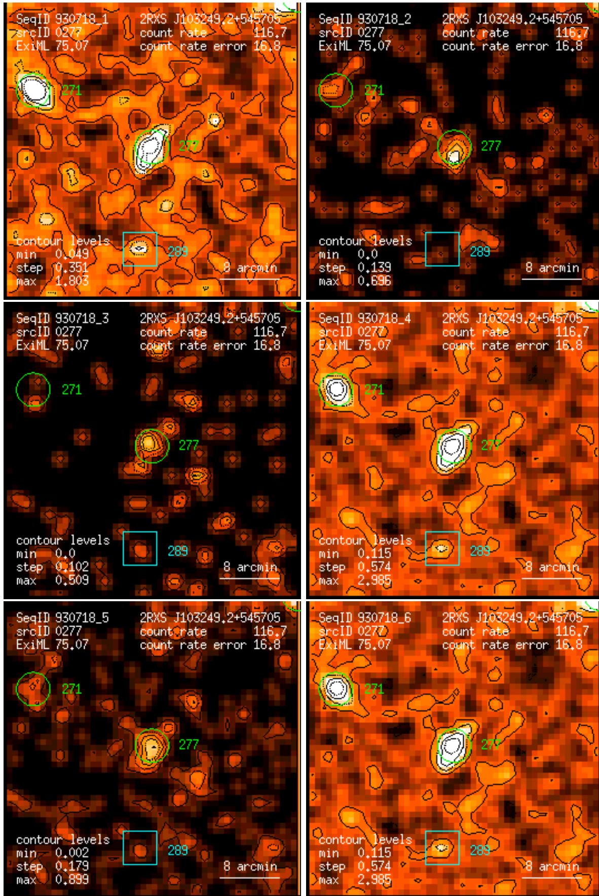
Figure 277: RASS 930718: detection 0277: band rate images, Gaussian filter: (1) PSPC channels 11 – 41, (2) 52 – 90, (3) 91 – 201, (4) 11 – 235, (5) 52 – 201, (6) 11 – 201. Broad band rates in counts/ks. Band rate contour levels in counts/ks/arcmin 2 .
