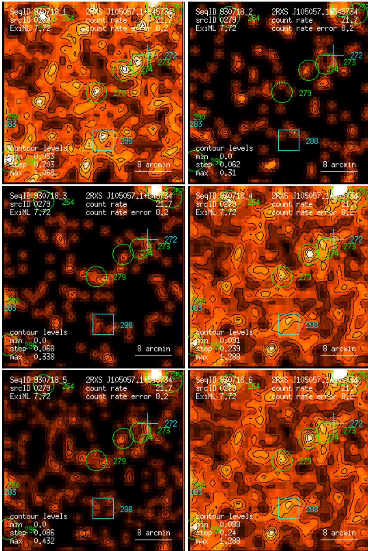
Figure 279: RASS 930718: detection 0279: band rate images, Gaussian filter: (1) PSPC channels 11 – 41, (2) 52 – 90, (3) 91 – 201, (4) 11 – 235, (5) 52 – 201, (6) 11 – 201. Broad band rates in counts/ks. Band rate contour levels in counts/ks/arcmin 2 .
