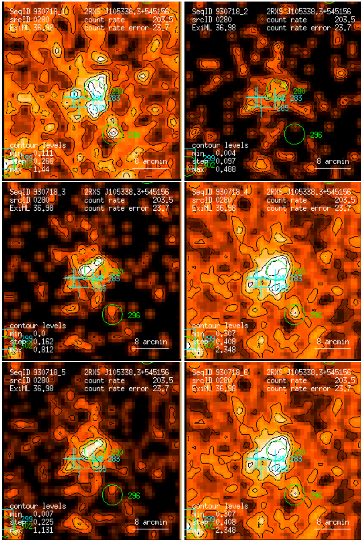
Figure 280: RASS 930718: detection 0280: band rate images, Gaussian filter: (1) PSPC channels 11 – 41, (2) 52 – 90, (3) 91 – 201, (4) 11 – 235, (5) 52 – 201, (6) 11 – 201. Broad band rates in counts/ks. Band rate contour levels in counts/ks/arcmin 2 .
