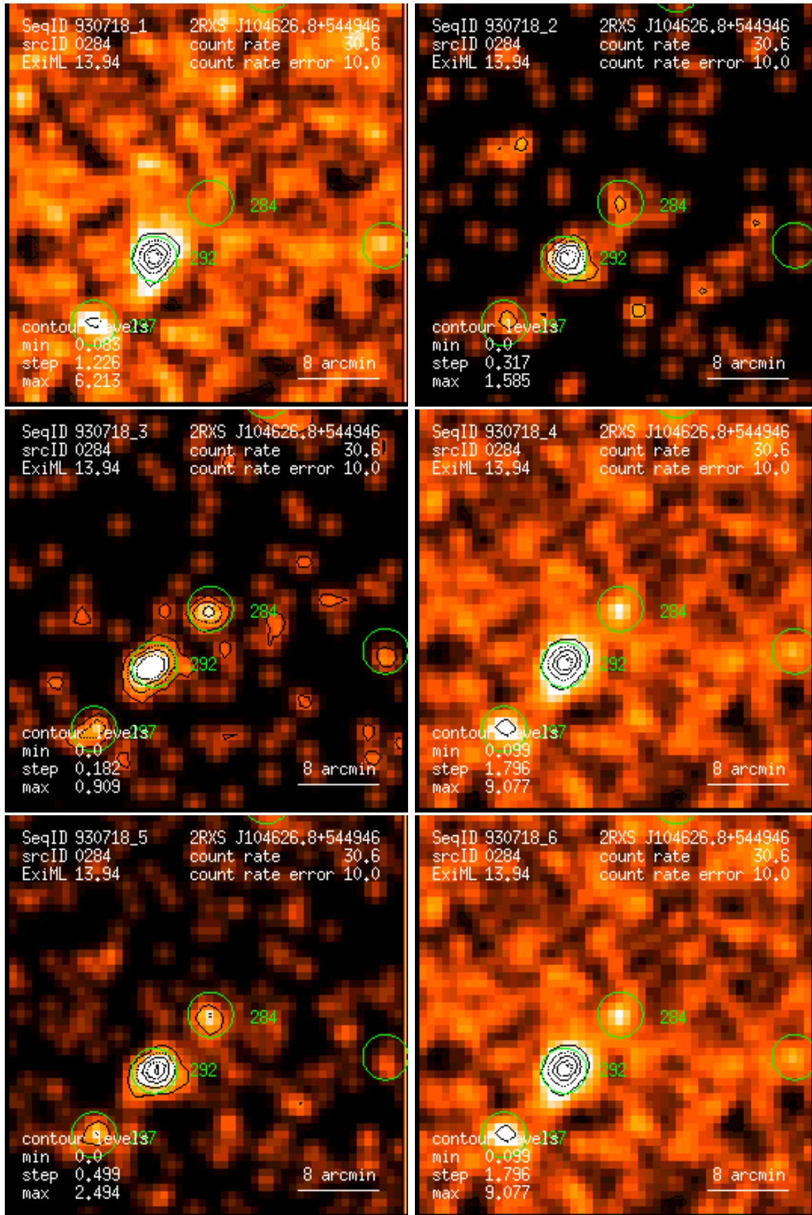
Figure 284: RASS 930718: detection 0284: band rate images, Gaussian filter: (1) PSPC channels 11 – 41, (2) 52 – 90, (3) 91 – 201, (4) 11 – 235, (5) 52 – 201, (6) 11 – 201. Broad band rates in counts/ks. Band rate contour levels in counts/ks/arcmin 2 .
