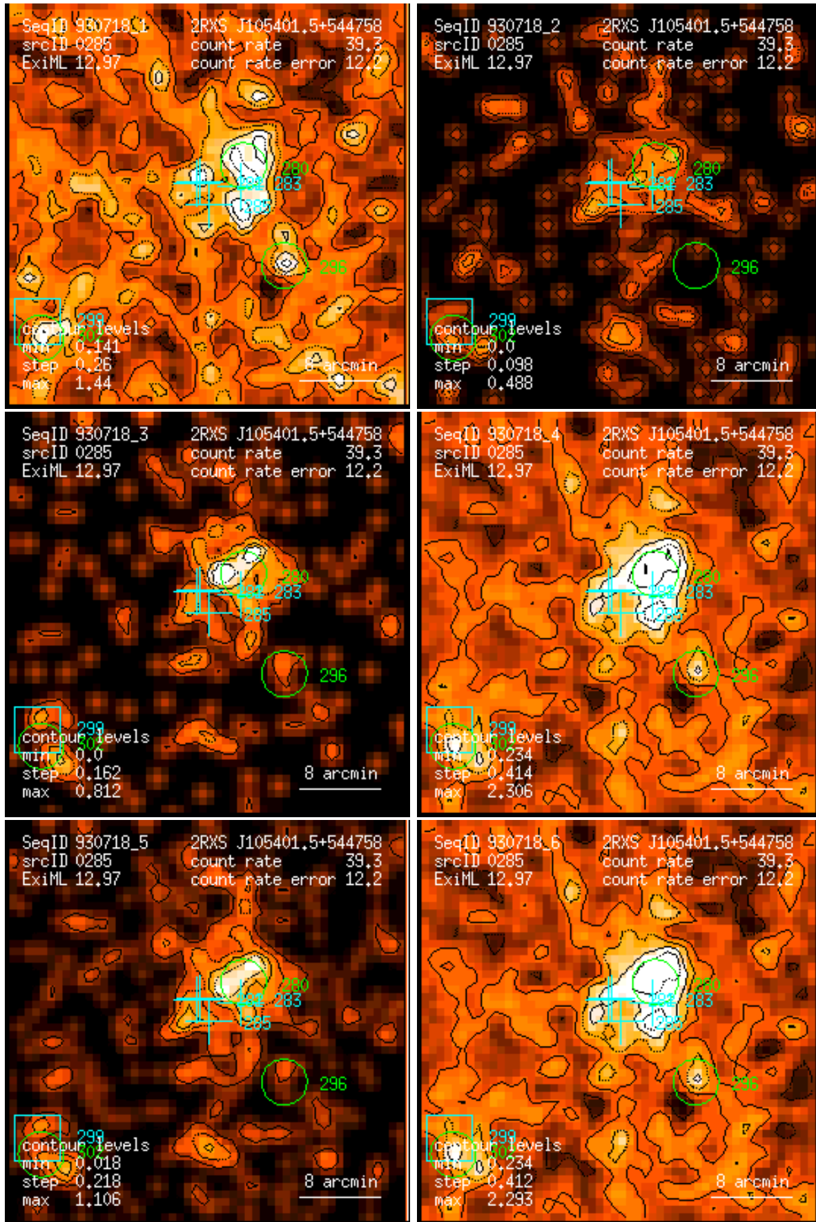
Figure 285: RASS 930718: detection 0285: band rate images, Gaussian filter: (1) PSPC channels 11 – 41, (2) 52 – 90, (3) 91 – 201, (4) 11 – 235, (5) 52 – 201, (6) 11 – 201. Broad band rates in counts/ks. Band rate contour levels in counts/ks/arcmin 2 .
