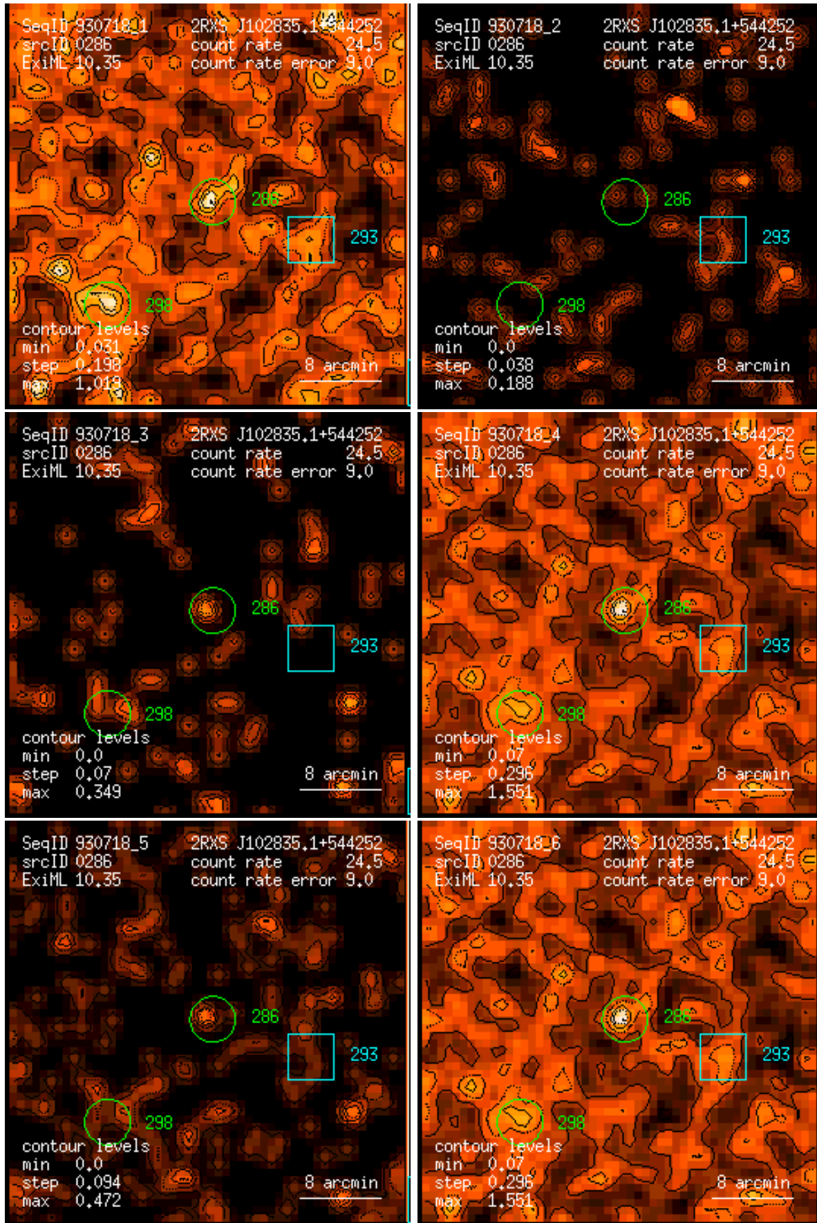
Figure 286: RASS 930718: detection 0286: band rate images, Gaussian filter: (1) PSPC channels 11 – 41, (2) 52 – 90, (3) 91 – 201, (4) 11 – 235, (5) 52 – 201, (6) 11 – 201. Broad band rates in counts/ks. Band rate contour levels in counts/ks/arcmin 2 .
