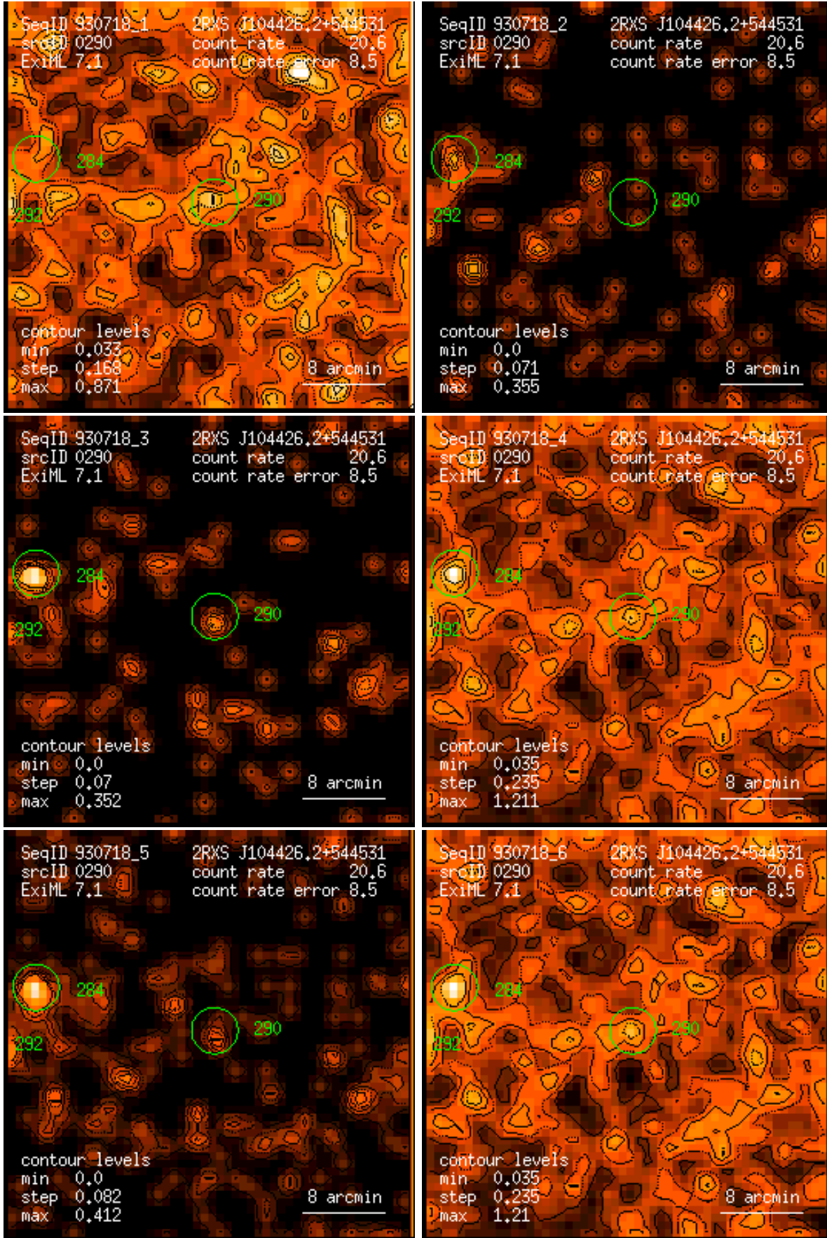
Figure 290: RASS 930718: detection 0290: band rate images, Gaussian filter: (1) PSPC channels 11 – 41, (2) 52 – 90, (3) 91 – 201, (4) 11 – 235, (5) 52 – 201, (6) 11 – 201. Broad band rates in counts/ks. Band rate contour levels in counts/ks/arcmin 2 .
