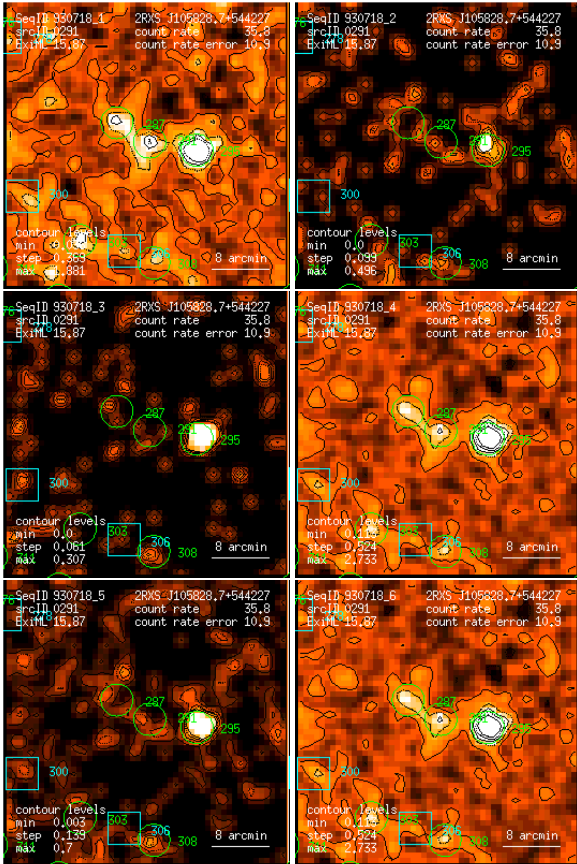
Figure 291: RASS 930718: detection 0291: band rate images, Gaussian filter: (1) PSPC channels 11 – 41, (2) 52 – 90, (3) 91 – 201, (4) 11 – 235, (5) 52 – 201, (6) 11 – 201. Broad band rates in counts/ks. Band rate contour levels in counts/ks/arcmin 2 .
