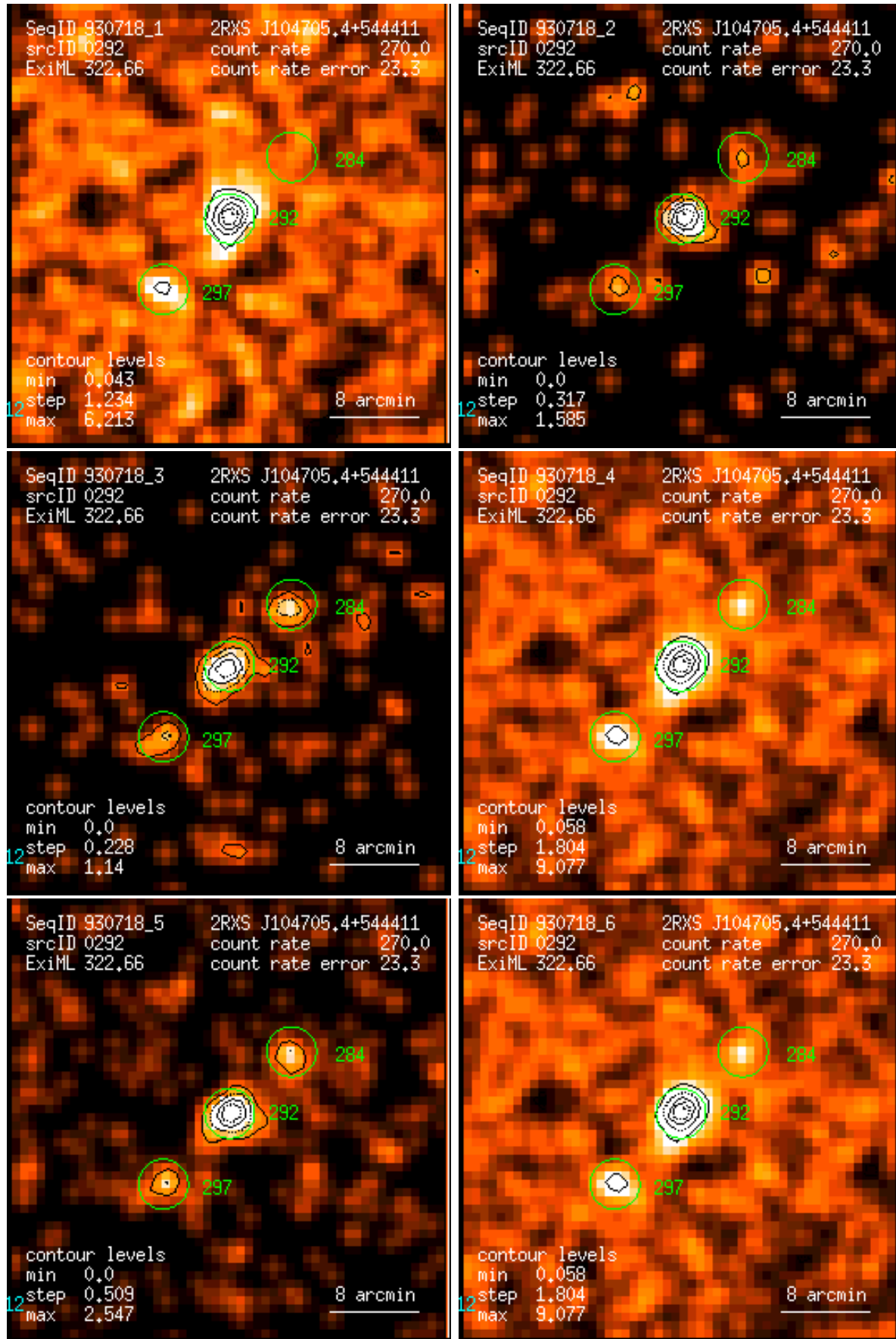
Figure 292: RASS 930718: detection 0292: band rate images, Gaussian filter: (1) PSPC channels 11 – 41, (2) 52 – 90, (3) 91 – 201, (4) 11 – 235, (5) 52 – 201, (6) 11 – 201. Broad band rates in counts/ks. Band rate contour levels in counts/ks/arcmin 2 .
