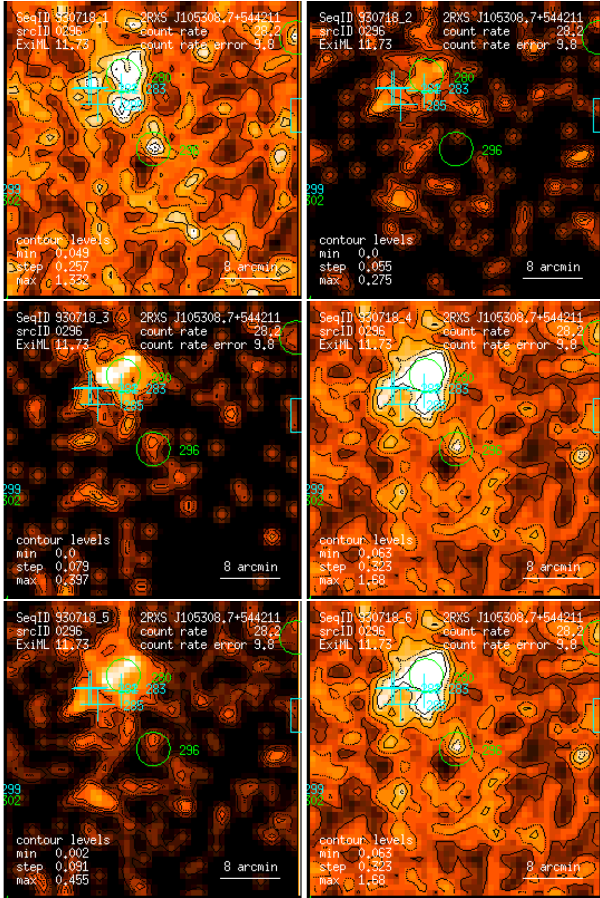
Figure 296: RASS 930718: detection 0296: band rate images, Gaussian filter: (1) PSPC channels 11 – 41, (2) 52 – 90, (3) 91 – 201, (4) 11 – 235, (5) 52 – 201, (6) 11 – 201. Broad band rates in counts/ks. Band rate contour levels in counts/ks/arcmin 2 .
