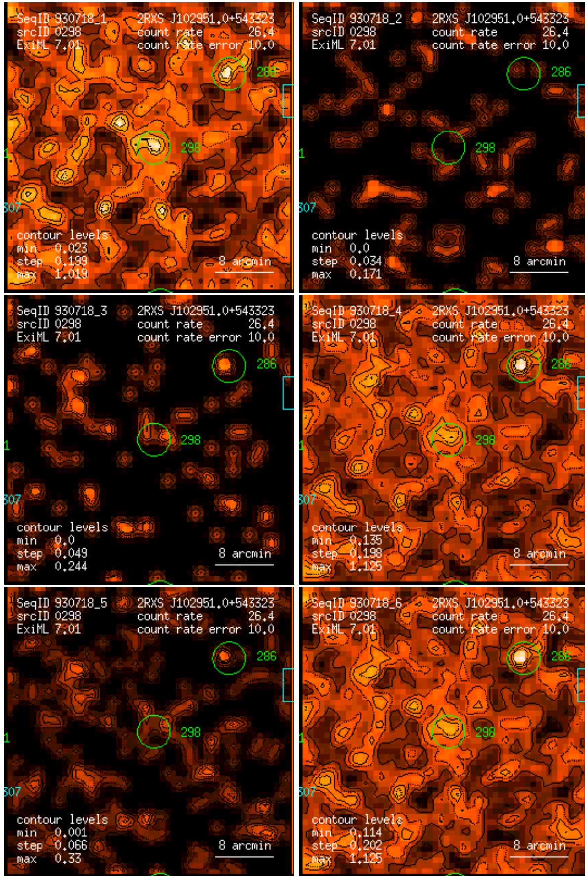
Figure 298: RASS 930718: detection 0298: band rate images, Gaussian filter: (1) PSPC channels 11 – 41, (2) 52 – 90, (3) 91 – 201, (4) 11 – 235, (5) 52 – 201, (6) 11 – 201. Broad band rates in counts/ks. Band rate contour levels in counts/ks/arcmin 2 .
