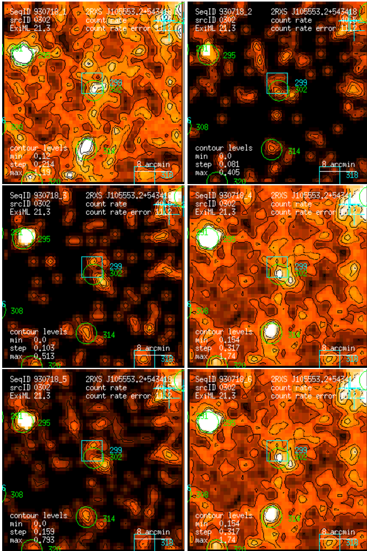
Figure 302: RASS 930718: detection 0302: band rate images, Gaussian filter: (1) PSPC channels 11 – 41, (2) 52 – 90, (3) 91 – 201, (4) 11 – 235, (5) 52 – 201, (6) 11 – 201. Broad band rates in counts/ks. Band rate contour levels in counts/ks/arcmin 2 .
