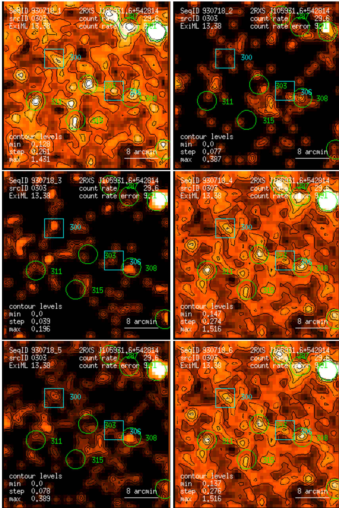
Figure 303: RASS 930718: detection 0303: band rate images, Gaussian filter: (1) PSPC channels 11 – 41, (2) 52 – 90, (3) 91 – 201, (4) 11 – 235, (5) 52 – 201, (6) 11 – 201. Broad band rates in counts/ks. Band rate contour levels in counts/ks/arcmin 2 .
