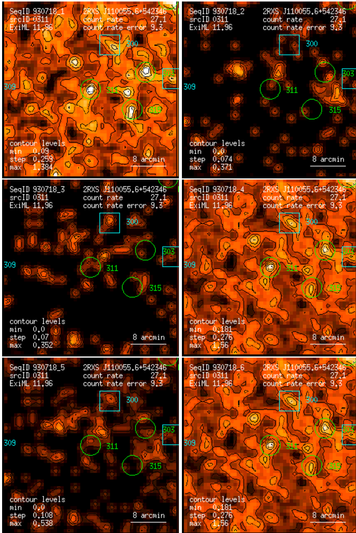
Figure 311: RASS 930718: detection 0311: band rate images, Gaussian filter: (1) PSPC channels 11 – 41, (2) 52 – 90, (3) 91 – 201, (4) 11 – 235, (5) 52 – 201, (6) 11 – 201. Broad band rates in counts/ks. Band rate contour levels in counts/ks/arcmin 2 .
