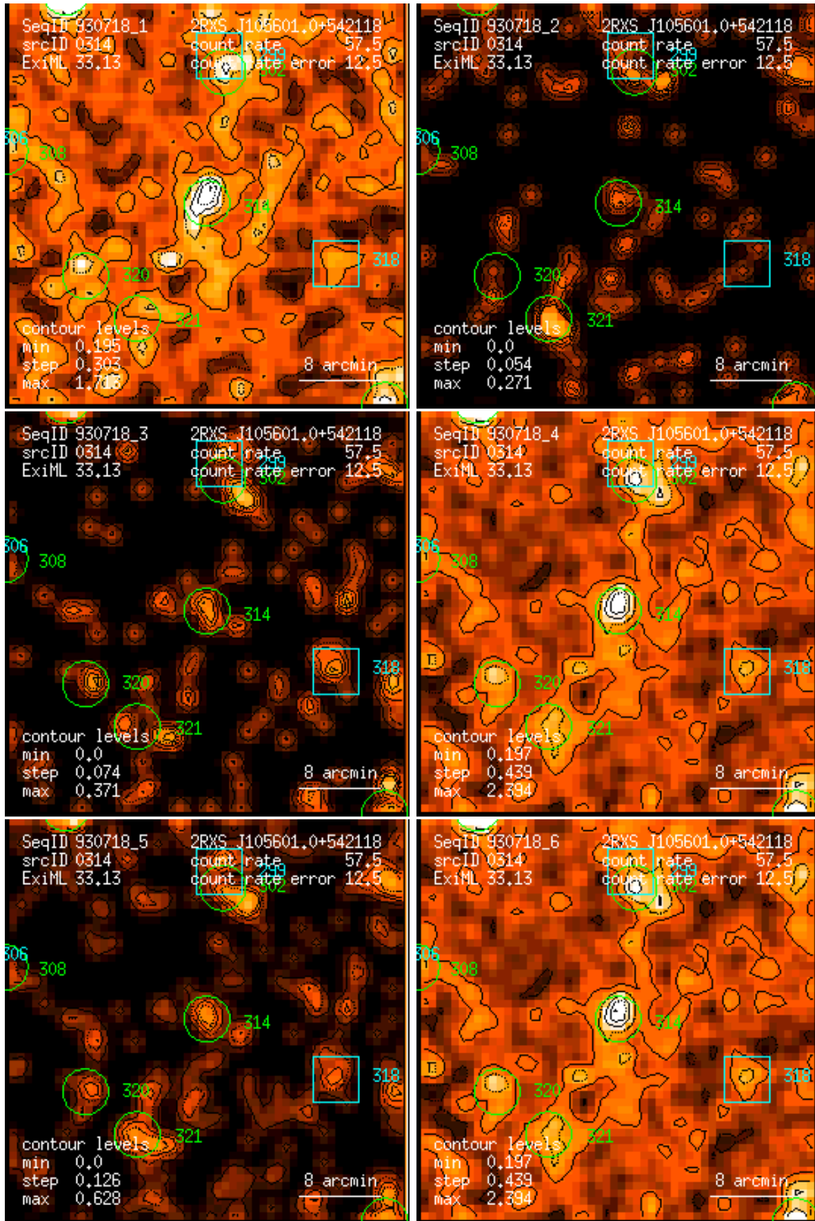
Figure 314: RASS 930718: detection 0314: band rate images, Gaussian filter: (1) PSPC channels 11 – 41, (2) 52 – 90, (3) 91 – 201, (4) 11 – 235, (5) 52 – 201, (6) 11 – 201. Broad band rates in counts/ks. Band rate contour levels in counts/ks/arcmin 2 .
