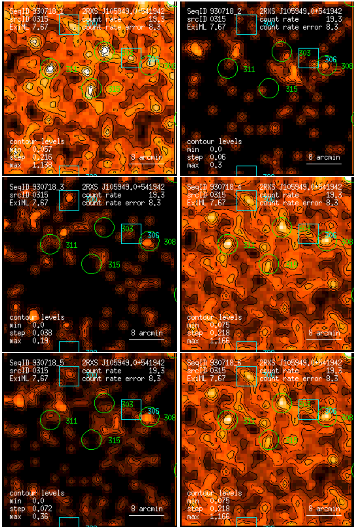
Figure 315: RASS 930718: detection 0315: band rate images, Gaussian filter: (1) PSPC channels 11 – 41, (2) 52 – 90, (3) 91 – 201, (4) 11 – 235, (5) 52 – 201, (6) 11 – 201. Broad band rates in counts/ks. Band rate contour levels in counts/ks/arcmin 2 .
