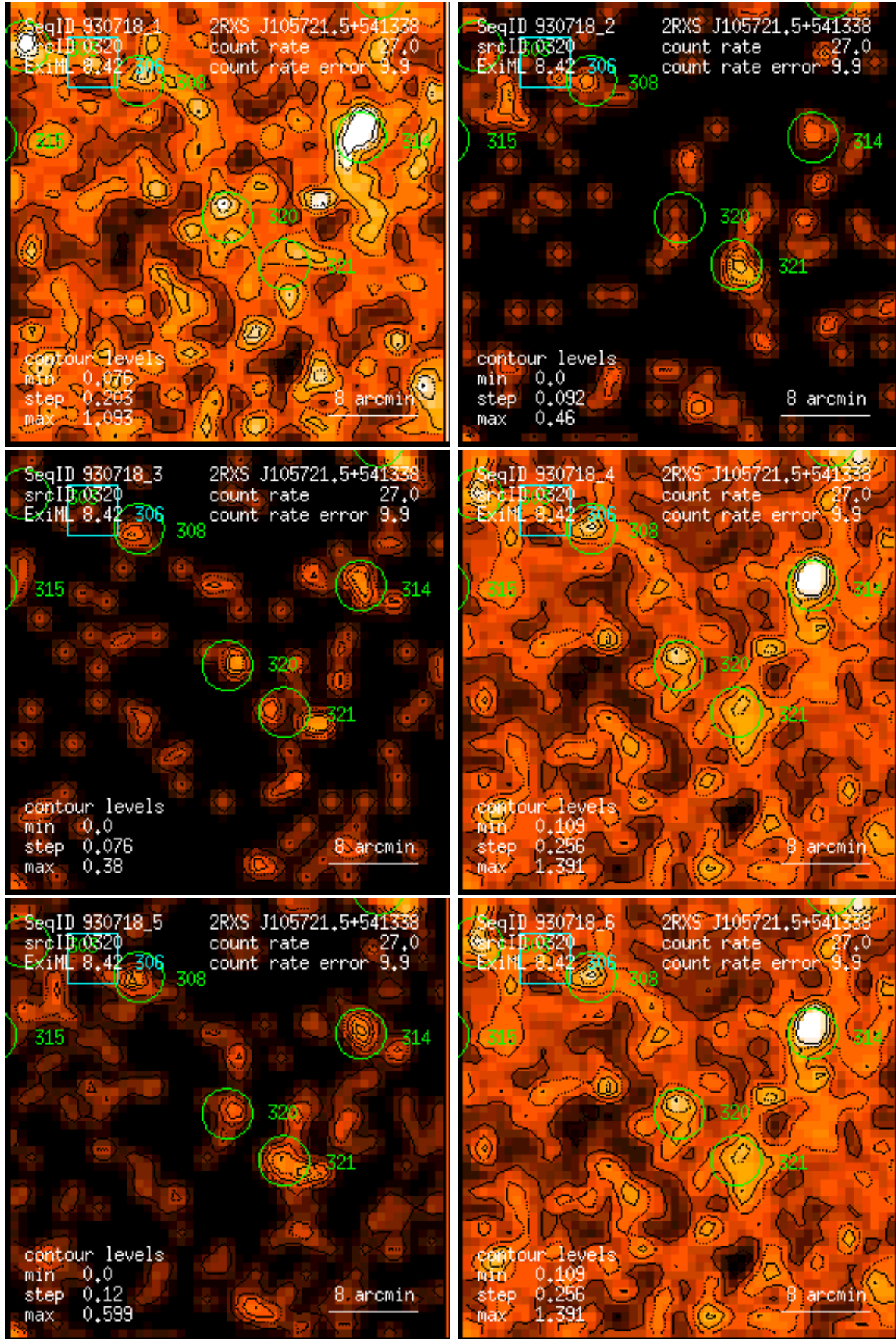
Figure 320: RASS 930718: detection 0320: band rate images, Gaussian filter: (1) PSPC channels 11 – 41, (2) 52 – 90, (3) 91 – 201, (4) 11 – 235, (5) 52 – 201, (6) 11 – 201. Broad band rates in counts/ks. Band rate contour levels in counts/ks/arcmin 2 .
