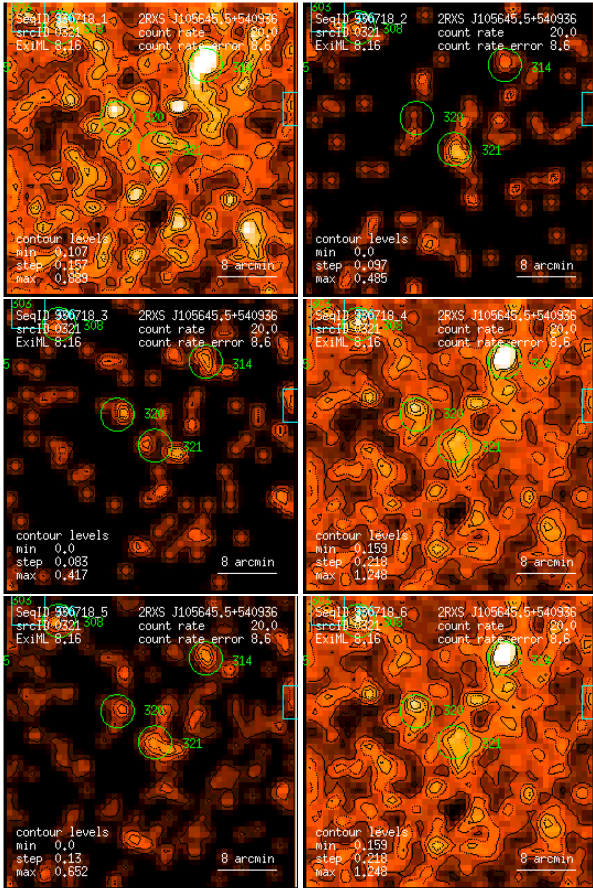
Figure 321: RASS 930718: detection 0321: band rate images, Gaussian filter: (1) PSPC channels 11 – 41, (2) 52 – 90, (3) 91 – 201, (4) 11 – 235, (5) 52 – 201, (6) 11 – 201. Broad band rates in counts/ks. Band rate contour levels in counts/ks/arcmin 2 .
