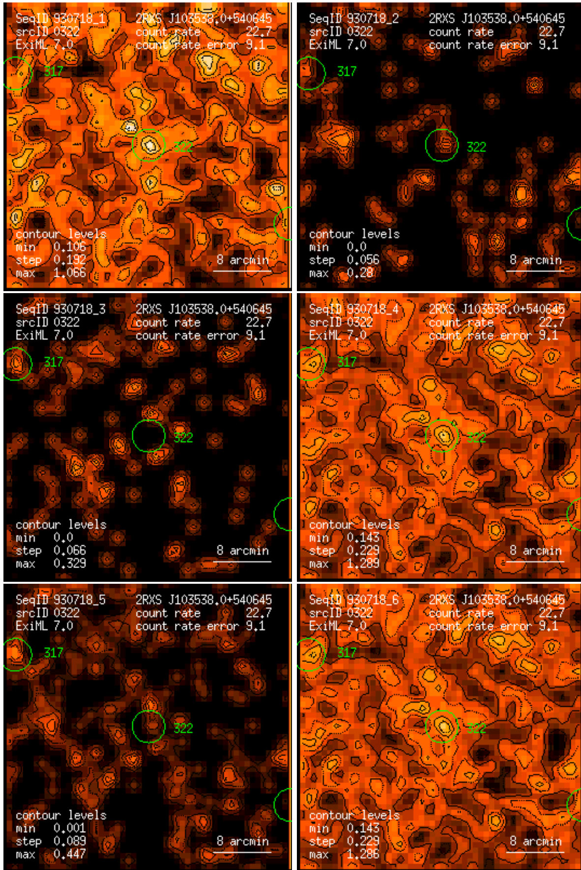
Figure 322: RASS 930718: detection 0322: band rate images, Gaussian filter: (1) PSPC channels 11 – 41, (2) 52 – 90, (3) 91 – 201, (4) 11 – 235, (5) 52 – 201, (6) 11 – 201. Broad band rates in counts/ks. Band rate contour levels in counts/ks/arcmin 2 .
