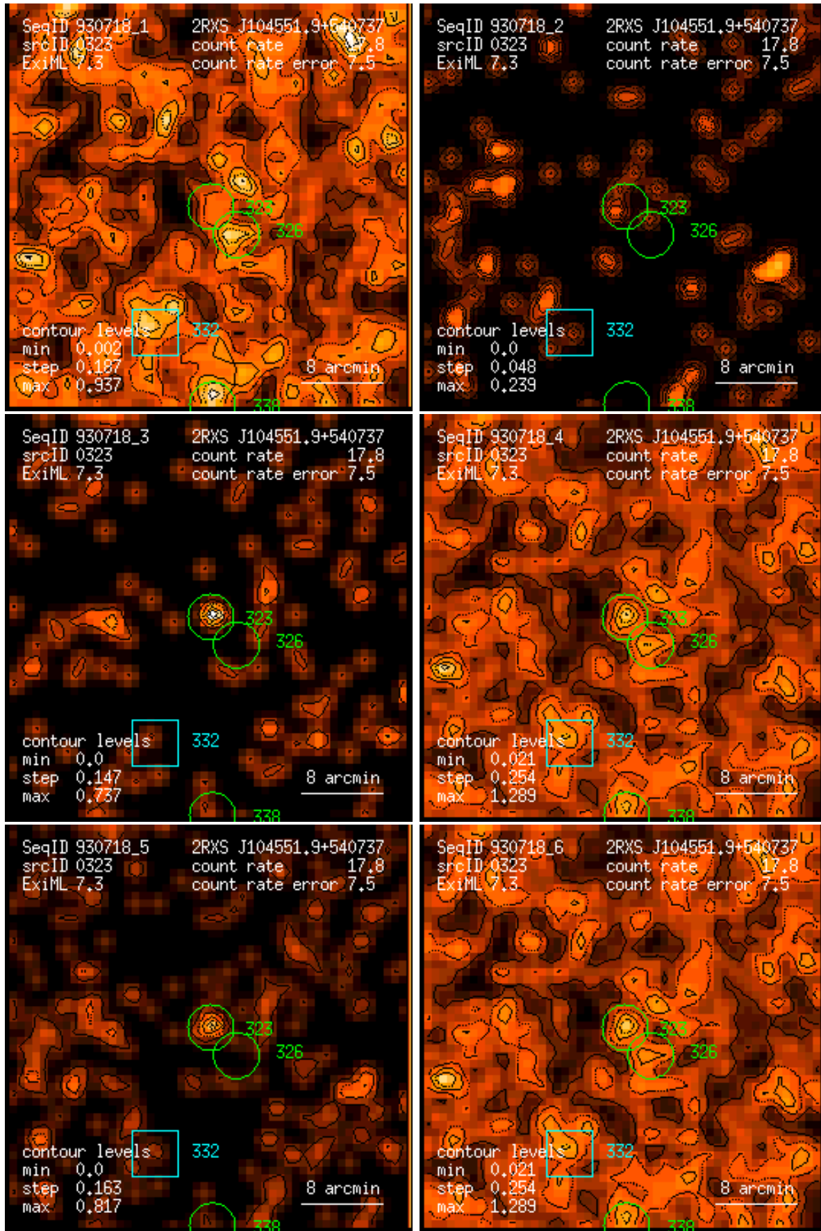
Figure 323: RASS 930718: detection 0323: band rate images, Gaussian filter: (1) PSPC channels 11 – 41, (2) 52 – 90, (3) 91 – 201, (4) 11 – 235, (5) 52 – 201, (6) 11 – 201. Broad band rates in counts/ks. Band rate contour levels in counts/ks/arcmin 2 .
