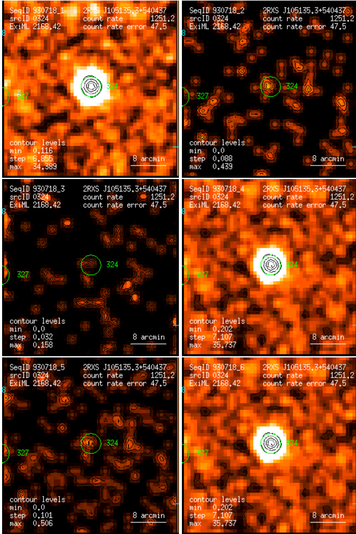
Figure 324: RASS 930718: detection 0324: band rate images, Gaussian filter: (1) PSPC channels 11 – 41, (2) 52 – 90, (3) 91 – 201, (4) 11 – 235, (5) 52 – 201, (6) 11 – 201. Broad band rates in counts/ks. Band rate contour levels in counts/ks/arcmin 2 .
