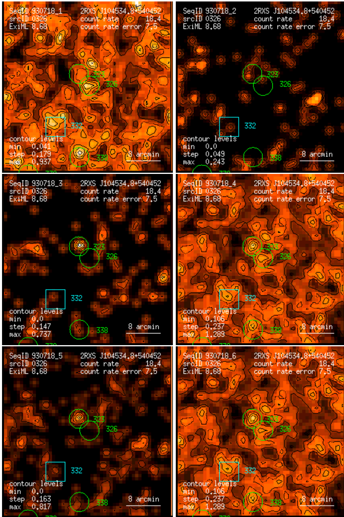
Figure 326: RASS 930718: detection 0326: band rate images, Gaussian filter: (1) PSPC channels 11 – 41, (2) 52 – 90, (3) 91 – 201, (4) 11 – 235, (5) 52 – 201, (6) 11 – 201. Broad band rates in counts/ks. Band rate contour levels in counts/ks/arcmin 2 .
