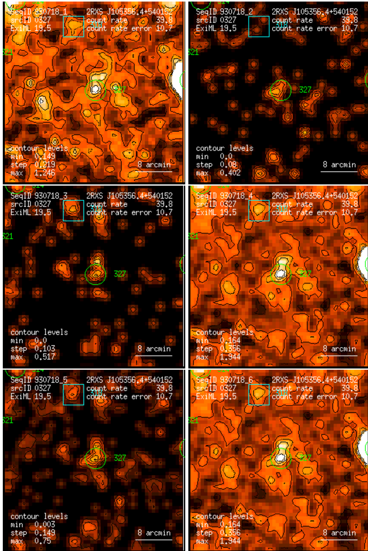
Figure 327: RASS 930718: detection 0327: band rate images, Gaussian filter: (1) PSPC channels 11 – 41, (2) 52 – 90, (3) 91 – 201, (4) 11 – 235, (5) 52 – 201, (6) 11 – 201. Broad band rates in counts/ks. Band rate contour levels in counts/ks/arcmin 2 .
