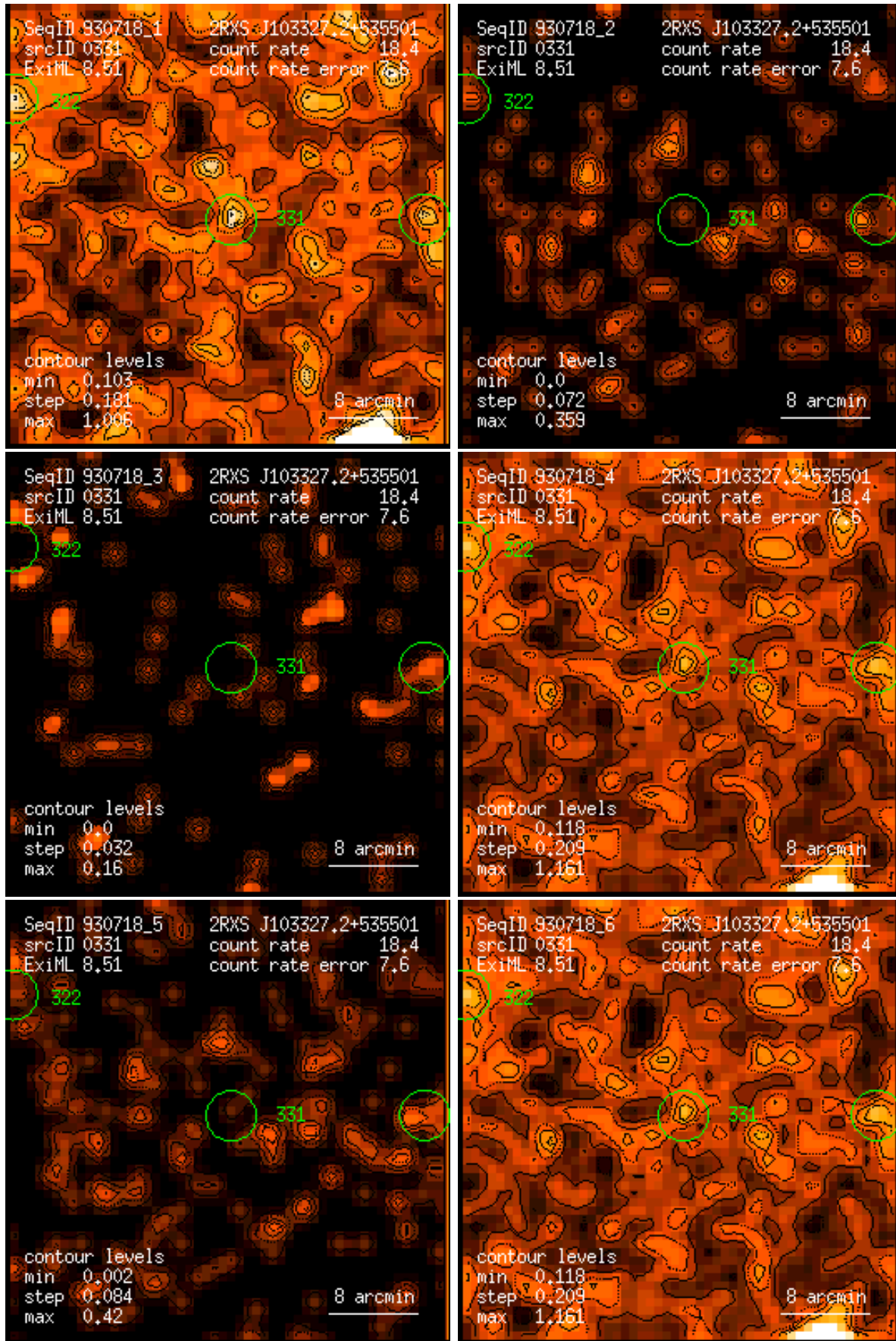
Figure 331: RASS 930718: detection 0331: band rate images, Gaussian filter: (1) PSPC channels 11 – 41, (2) 52 – 90, (3) 91 – 201, (4) 11 – 235, (5) 52 – 201, (6) 11 – 201. Broad band rates in counts/ks. Band rate contour levels in counts/ks/arcmin 2 .
