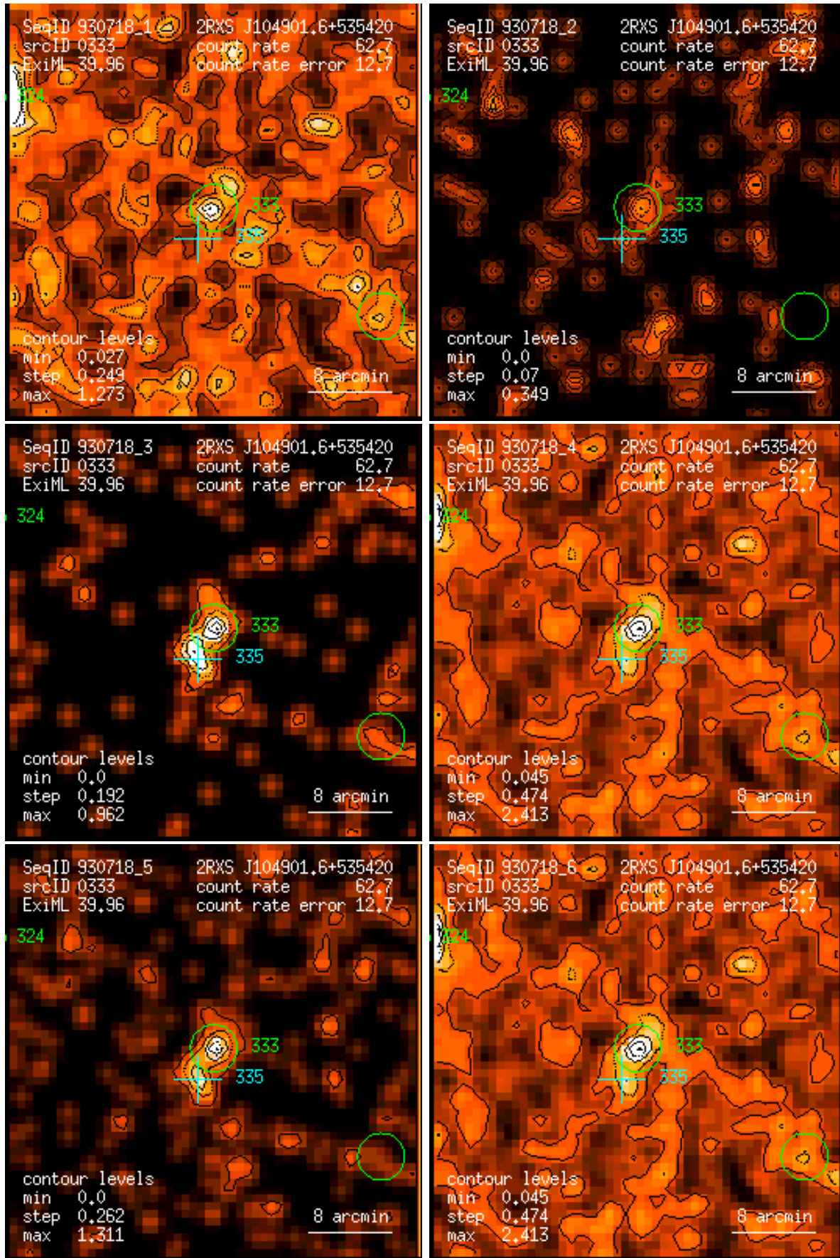
Figure 333: RASS 930718: detection 0333: band rate images, Gaussian filter: (1) PSPC channels 11 – 41, (2) 52 – 90, (3) 91 – 201, (4) 11 – 235, (5) 52 – 201, (6) 11 – 201. Broad band rates in counts/ks. Band rate contour levels in counts/ks/arcmin 2 .
