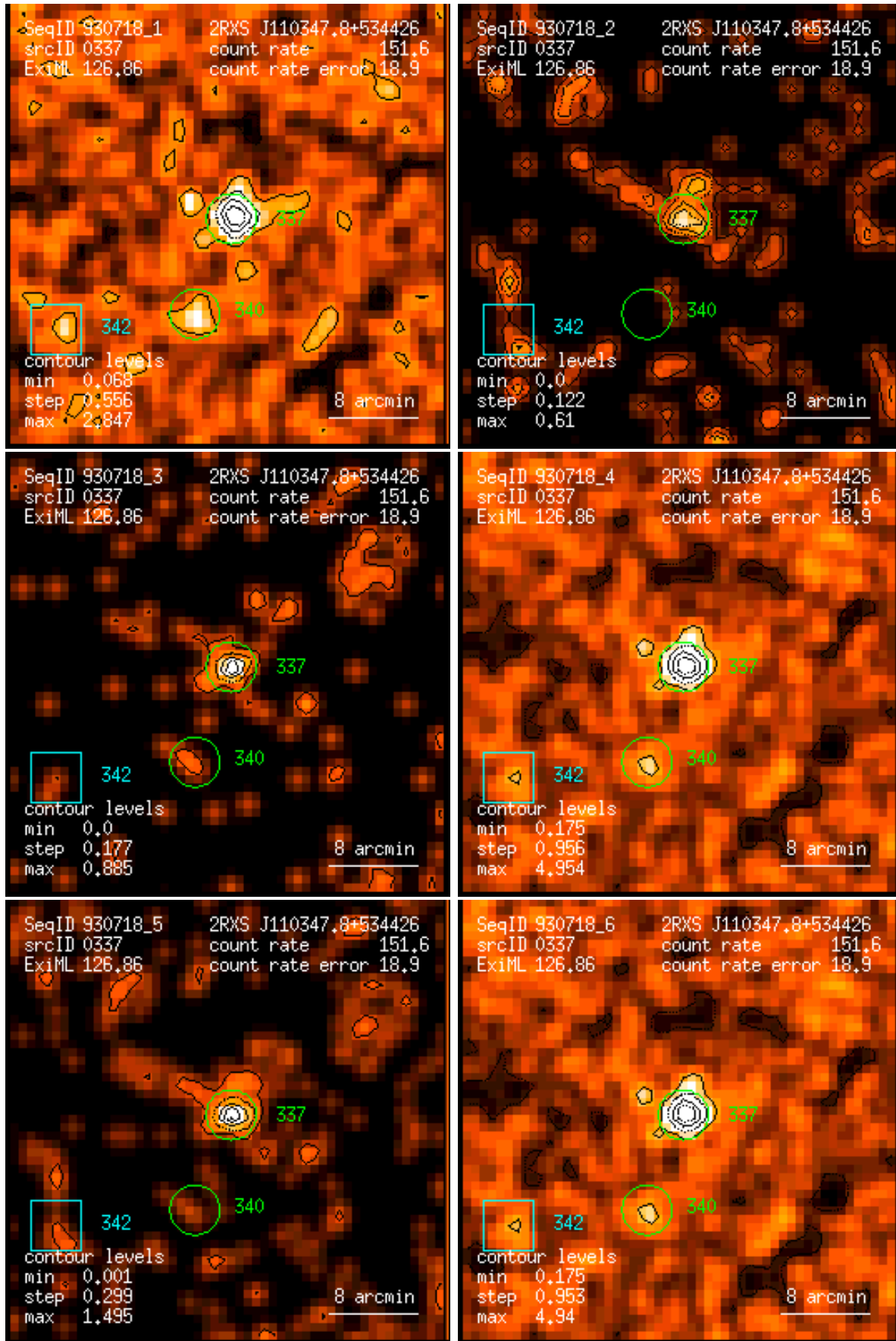
Figure 337: RASS 930718: detection 0337: band rate images, Gaussian filter: (1) PSPC channels 11 – 41, (2) 52 – 90, (3) 91 – 201, (4) 11 – 235, (5) 52 – 201, (6) 11 – 201. Broad band rates in counts/ks. Band rate contour levels in counts/ks/arcmin 2 .
