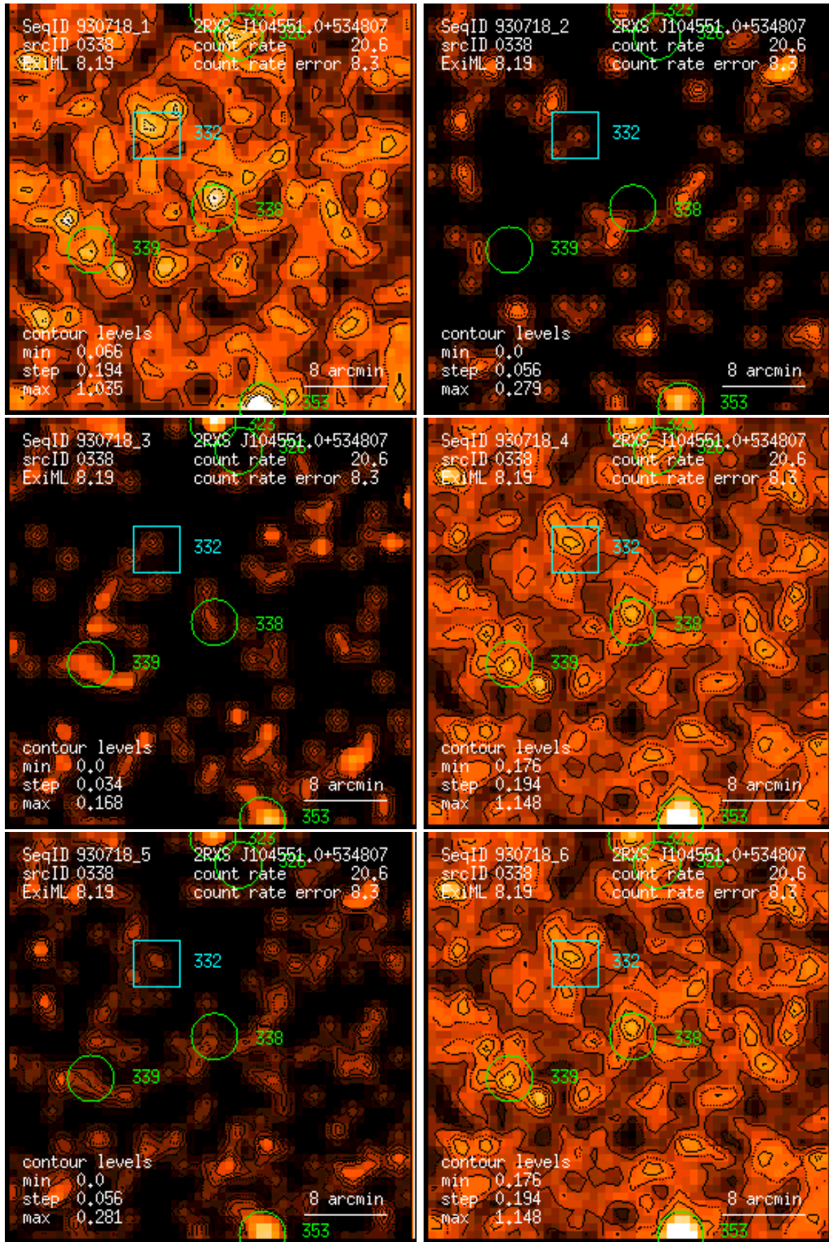
Figure 338: RASS 930718: detection 0338: band rate images, Gaussian filter: (1) PSPC channels 11 – 41, (2) 52 – 90, (3) 91 – 201, (4) 11 – 235, (5) 52 – 201, (6) 11 – 201. Broad band rates in counts/ks. Band rate contour levels in counts/ks/arcmin 2 .
