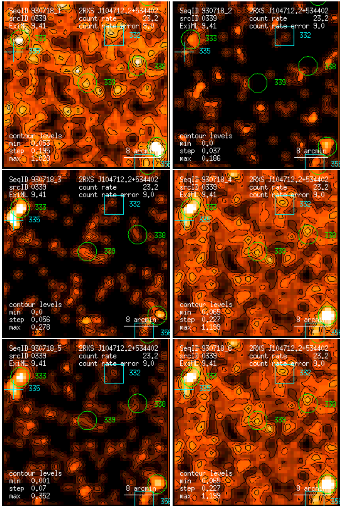
Figure 339: RASS 930718: detection 0339: band rate images, Gaussian filter: (1) PSPPC channels 11 – 41, (2) 52 – 90, (3) 91 – 201, (4) 11 – 235, (5) 52 – 201, (6) 11 – 201. Broad band rates in counts/ks. Band rate contour levels in counts/ks/arcmin 2 .
