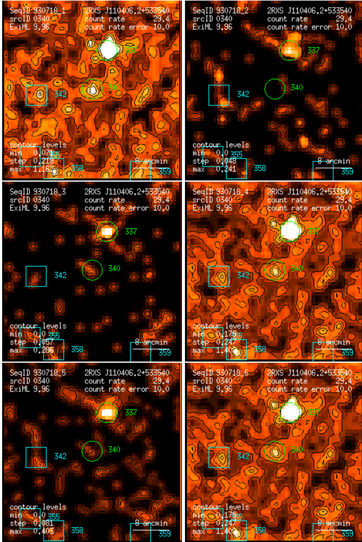
Figure 340: RASS 930718: detection 0340: band rate images, Gaussian filter: (1) PSPC channels 11 – 41, (2) 52 – 90, (3) 91 – 201, (4) 11 – 235, (5) 52 – 201, (6) 11 – 201. Broad band rates in counts/ks. Band rate contour levels in counts/ks/arcmin 2 .
