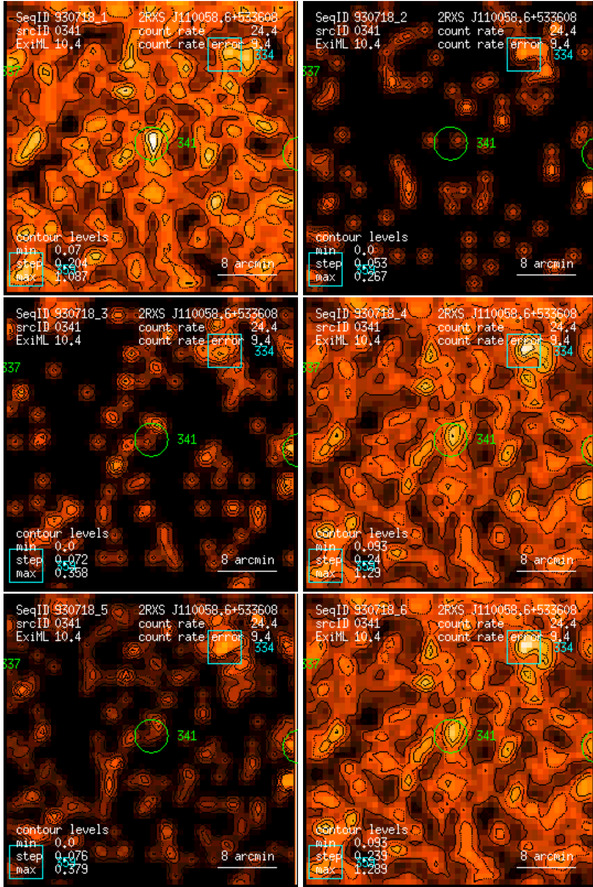
Figure 341: RASS 930718: detection 0341: band rate images, Gaussian filter: (1) PSPC channels 11 – 41, (2) 52 – 90, (3) 91 – 201, (4) 11 – 235, (5) 52 – 201, (6) 11 – 201. Broad band rates in counts/ks. Band rate contour levels in counts/ks/arcmin 2 .
